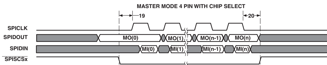
Figure 9-35 SPI Additional Timings for 4-Pin Master Mode with Chip Select Option
