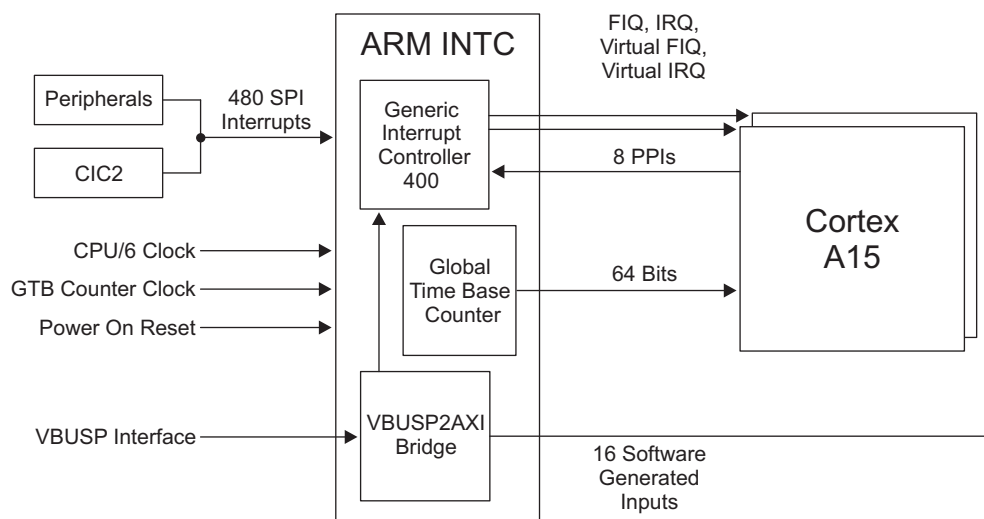
Figure 3-2 ARM Interrupt Controller for Two Cortex-A15 Processor Cores
