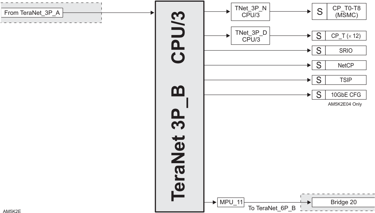
Figure 6-5 TeraNet 3P_B
