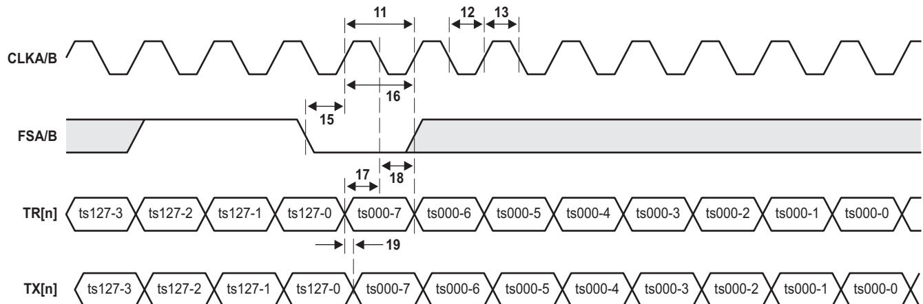
Figure 9-51 TSIP 1x Timing Diagram (1)
