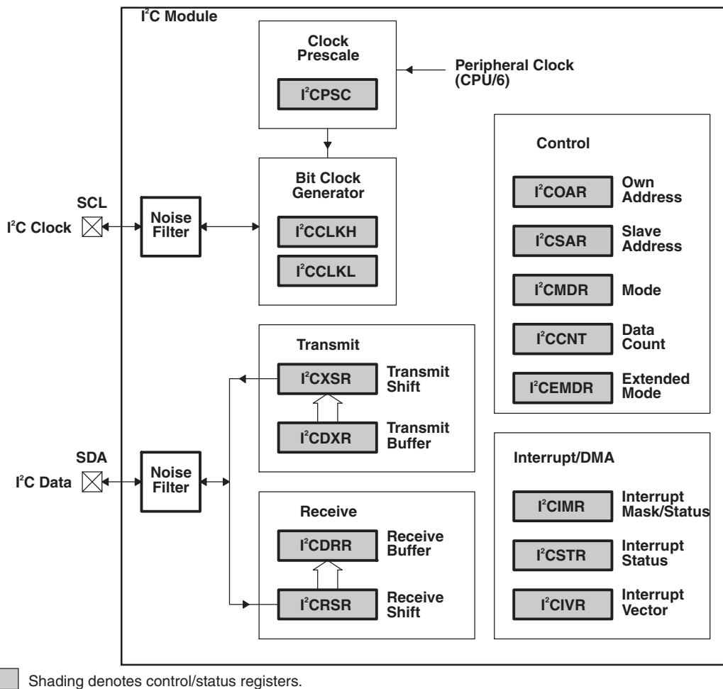
Figure 9-31 I 2 C Module Block Diagram
