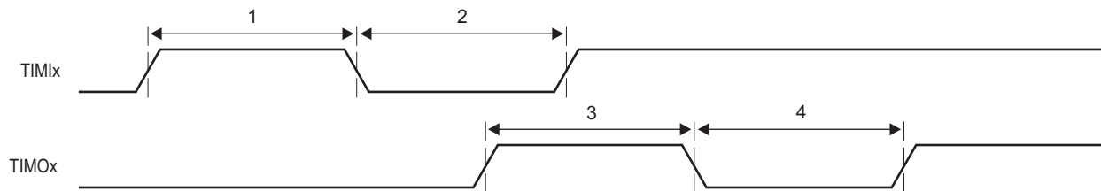
Figure 9-48 Timer Timing
