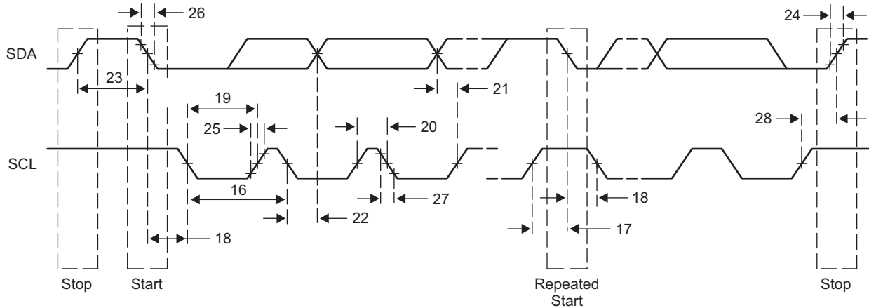
Figure 9-33 I 2 C Transmit Timings
