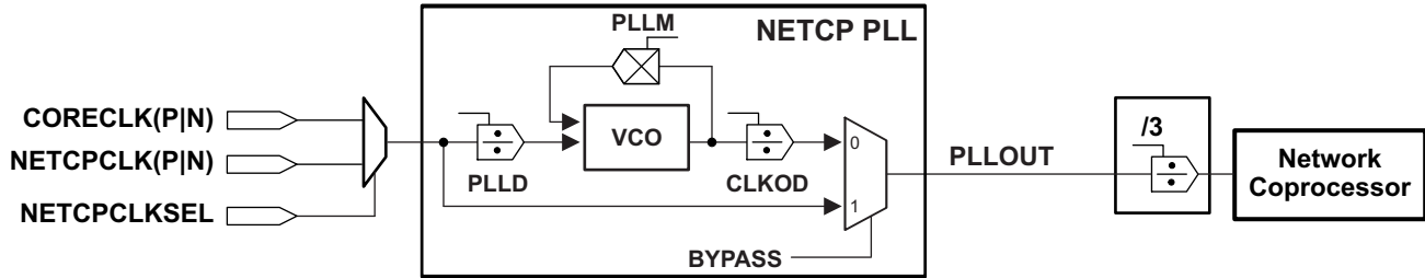
Figure 9-27 NETCP PLL Block Diagram
