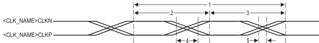
Figure 9-20 Core PLL Transition Time
