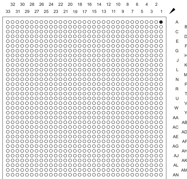
Figure 4-1 ABD 1089-PIN BGA Package (Bottom View)
