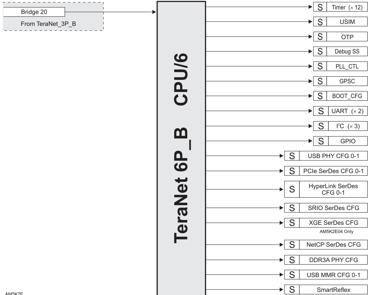
Figure 6-6 TeraNet 6P_B
