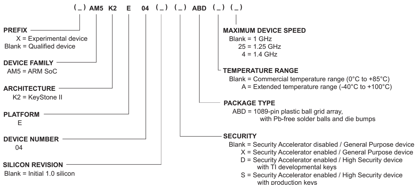
Figure 2-2 Device Nomenclature for AM5K2E04
