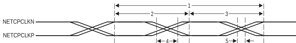
Figure 9-30 NETCP PLL Timing
