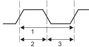
Figure 9-37 HyperLink Station Management Transmit Timing
