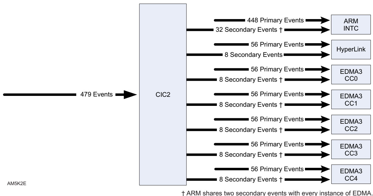
Figure 5-4 Interrupt Topology for AM5K2E04/02
