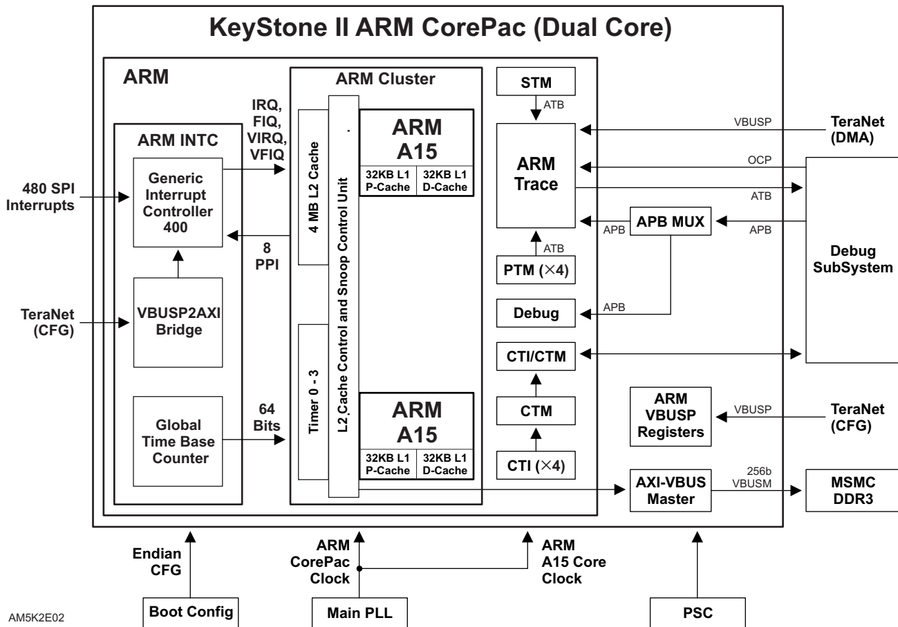
Figure 3-1 ARM CorePac Block Diagram
