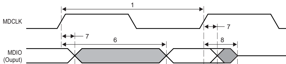
Figure 9-47 MDIO Output Timing
