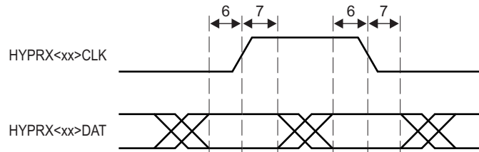
Figure 9-38 HyperLink Station Management Receive Timing
