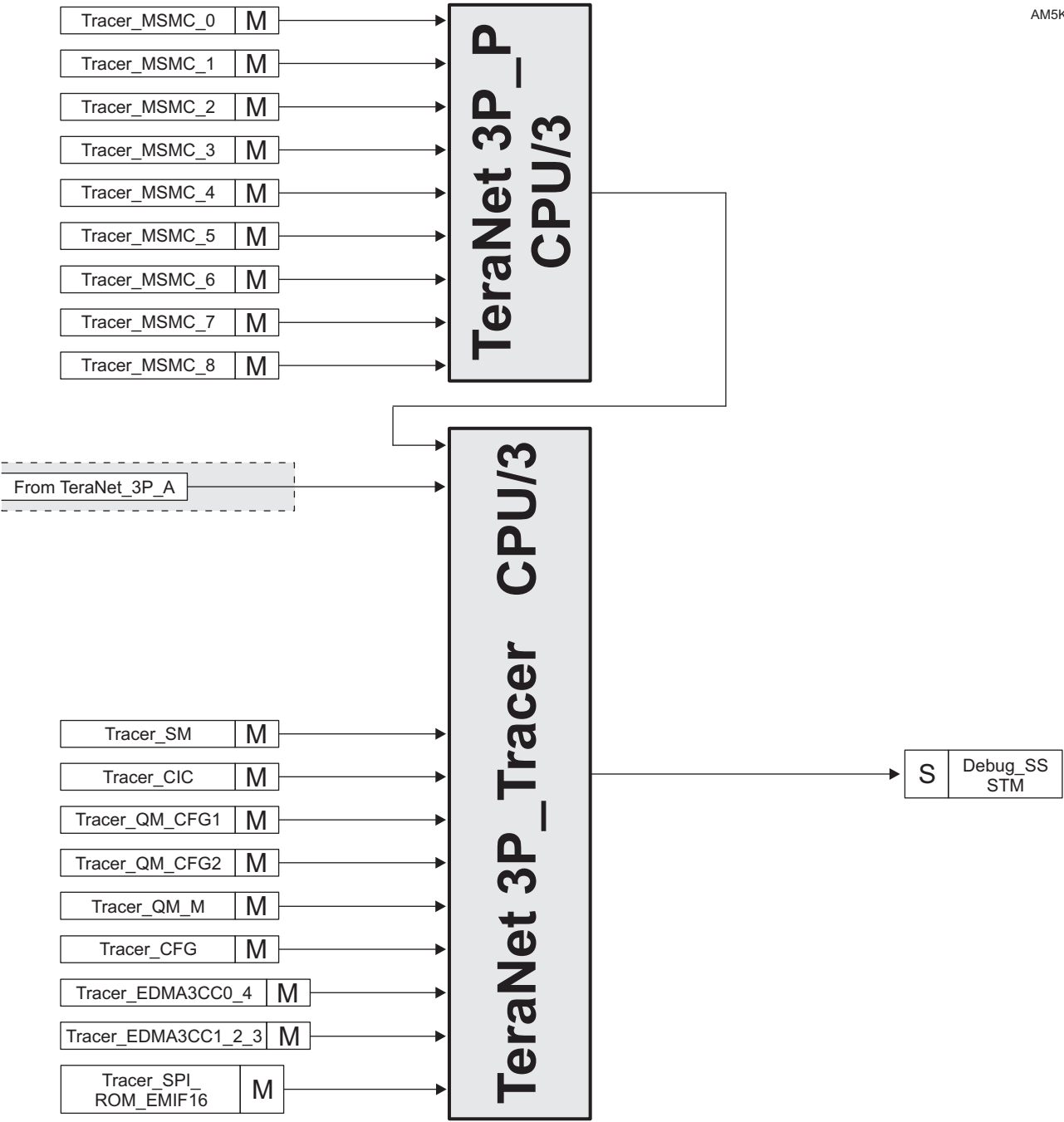
Figure 6-7 TeraNet 3P_Tracer
