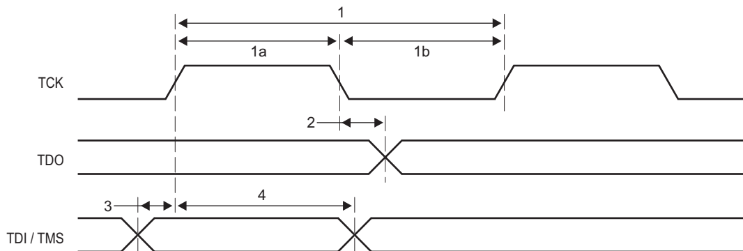
Figure 9-57 JTAG Test-Port Timing
