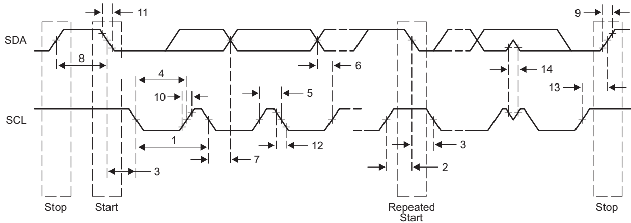
Figure 9-32 I 2 C Receive Timings
