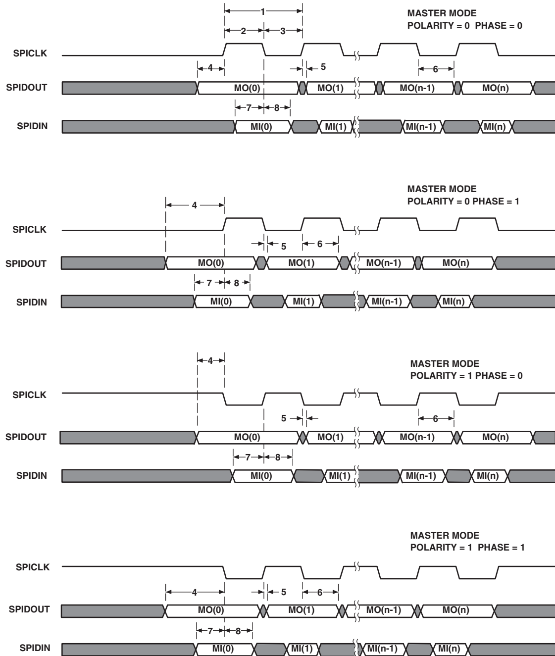
Figure 9-34 SPI Master Mode Timing Diagrams — Base Timings for 3-Pin Mode
