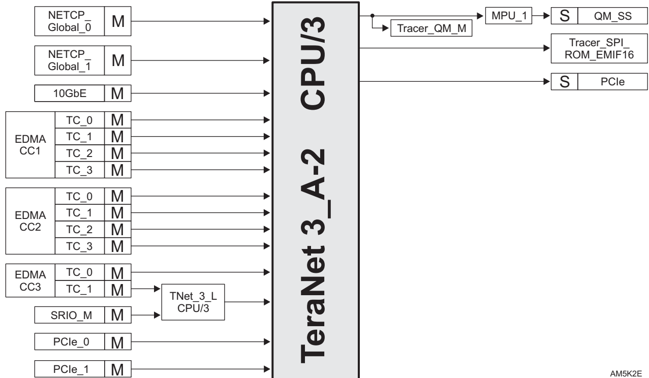
Figure 6-2 TeraNet 3_A-2
