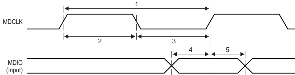
Figure 9-46 MDIO Input Timing
