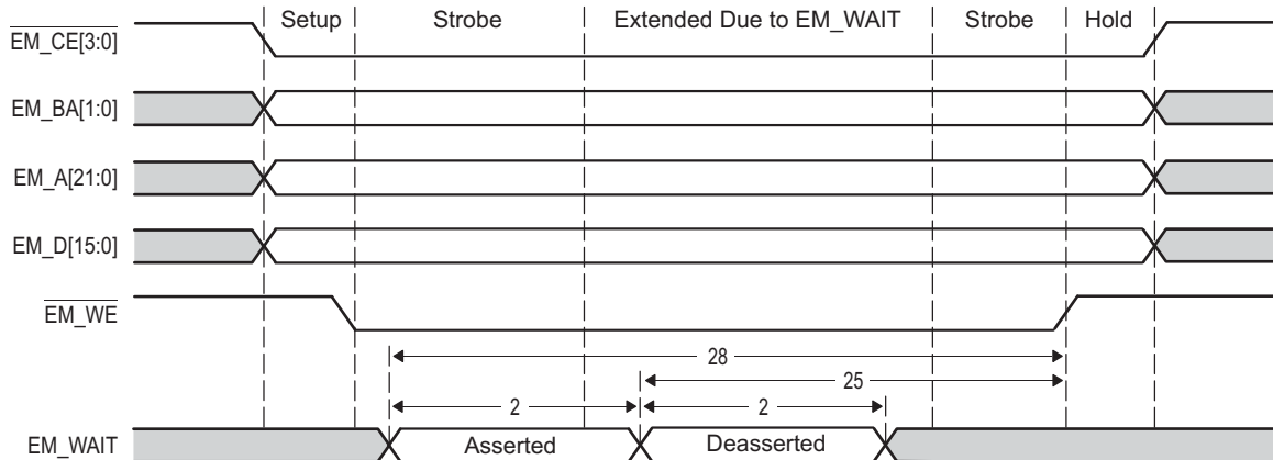
Figure 9-55 EMIF16 EM_WAIT Write Timing Diagram
