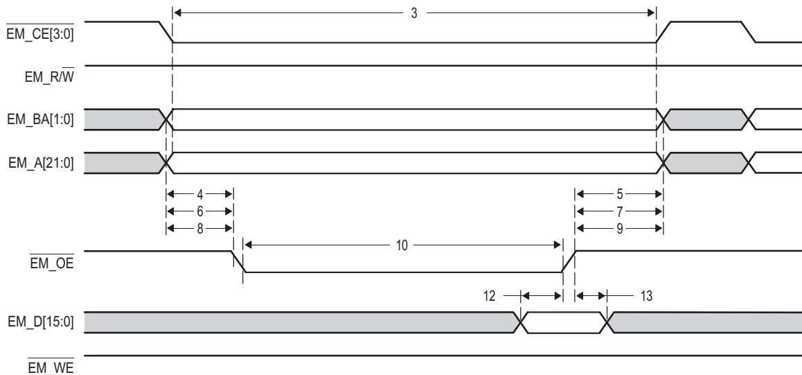
Figure 9-52 EMIF16 Asynchronous Memory Read Timing Diagram
