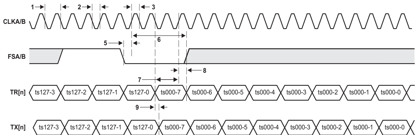
Figure 9-50 TSIP 2x Timing Diagram (1)
