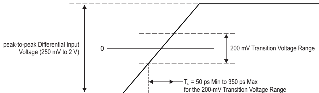
Figure 9-21 HYP0CLK, HYP1CLK, XF1CLK and PCIECLK Rise and Fall Times
