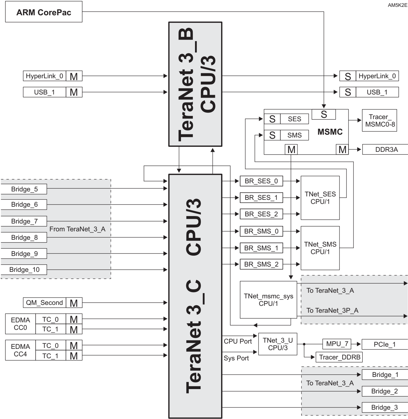
Figure 6-3 TeraNet 3_C
