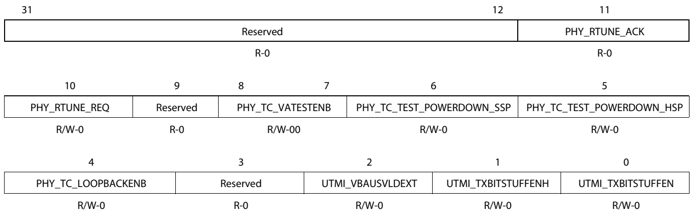
Figure 7-34 USB_PHY_CTL0 Register
