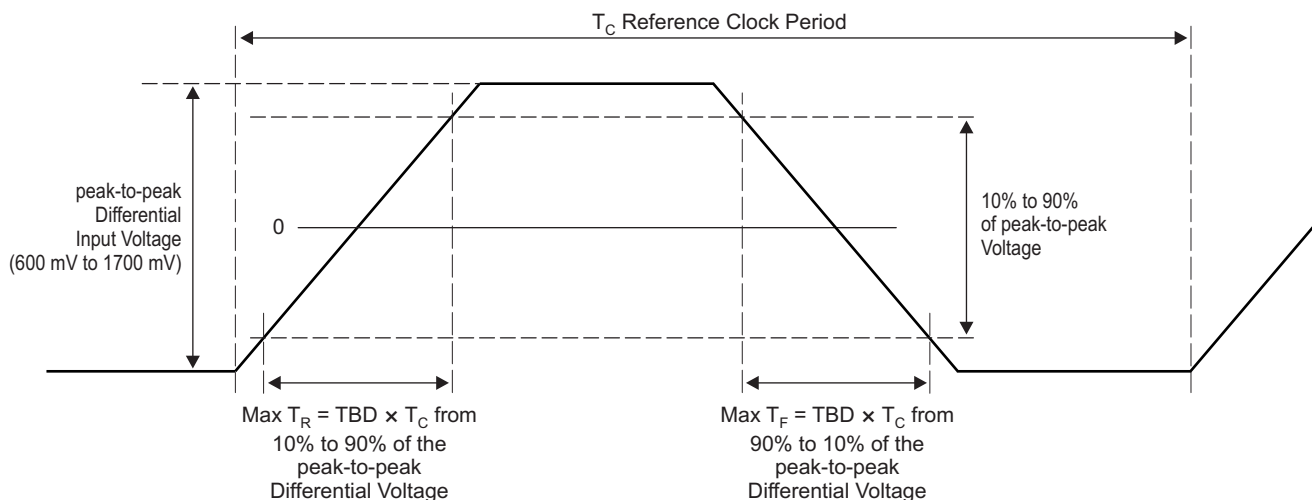
Figure 9-22 USBCLK Rise and Fall Times
