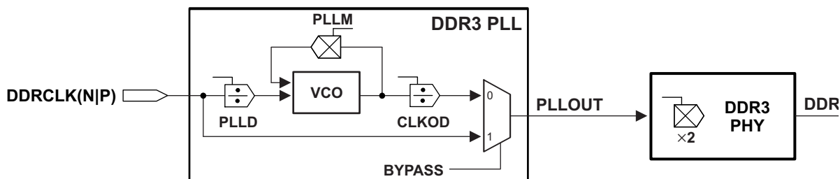
Figure 9-23 DDR3A PLL Block Diagram
