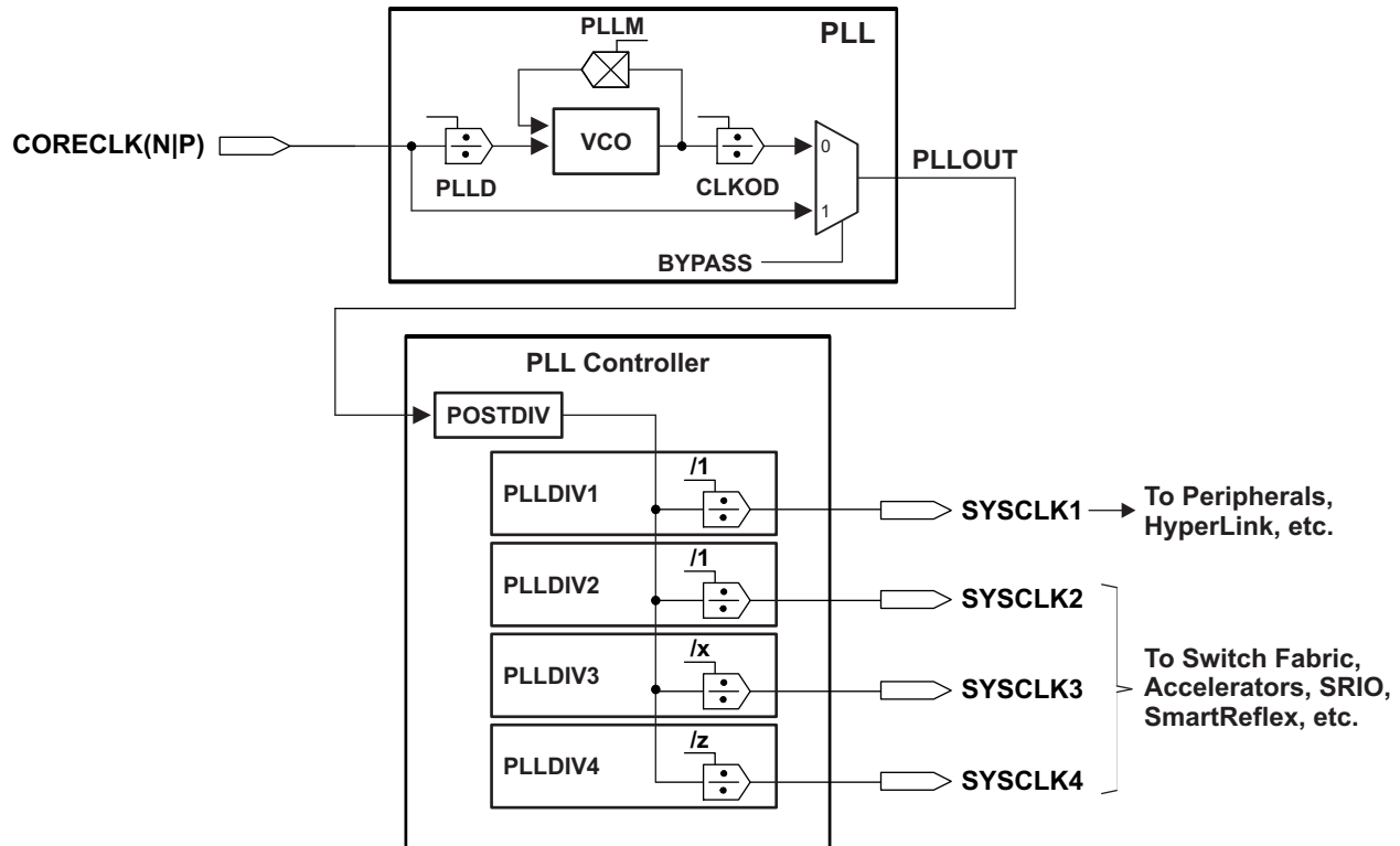
Figure 9-7 Core PLL and PLL Controller
