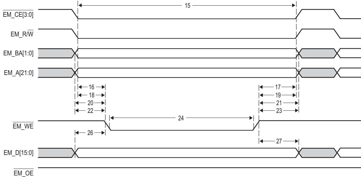
Figure 9-54 EMIF16 EM_WAIT Read Timing Diagram
