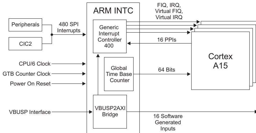
Figure 3-3 ARM Interrupt Controller for Four Cortex-A15 Processor Cores
