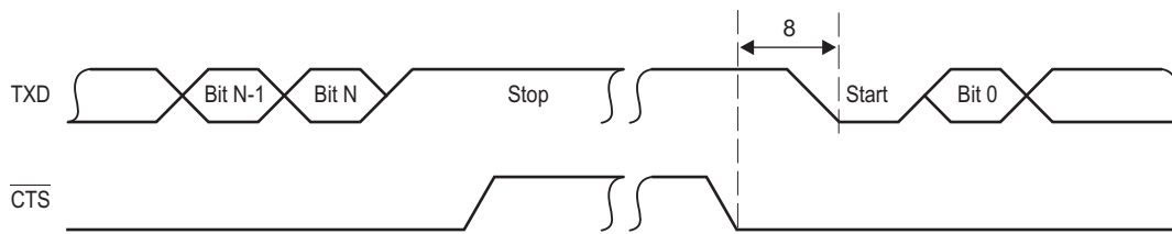
Figure 9-40 UART CTS (Clear-to-Send Input) — Autoflow Timing Waveform
