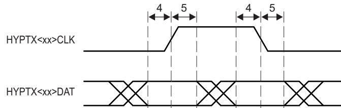
Figure 9-37 HyperLink Station Management Transmit Timing
