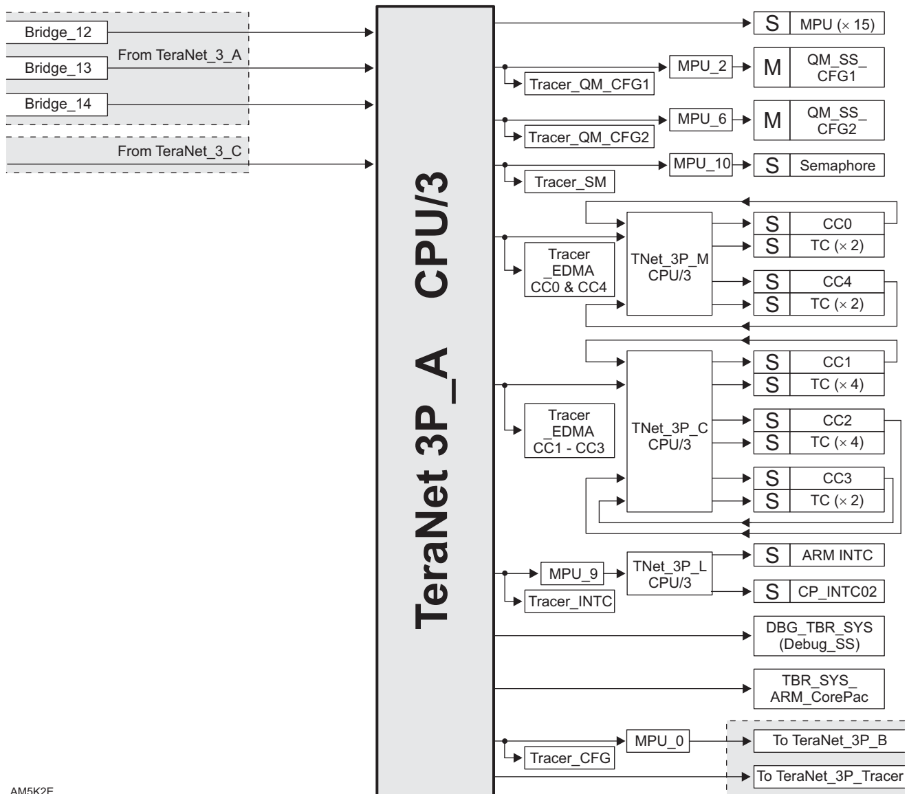
Figure 6-4 TeraNet 3P_A
