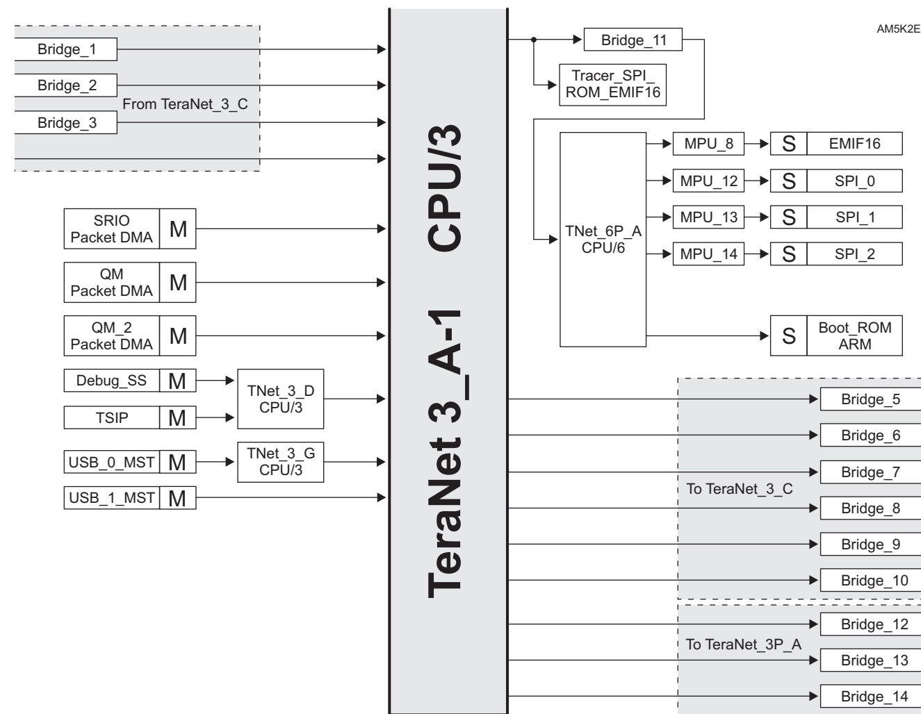
Figure 6-1 TeraNet 3_A-1
