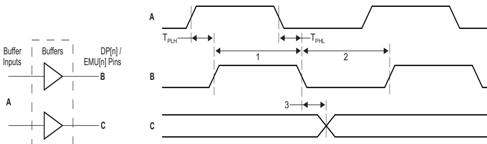
Figure 9-56 Trace Timing
