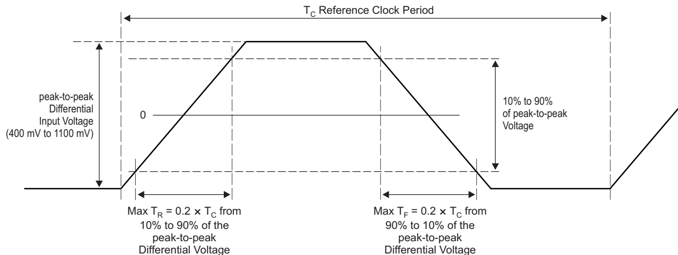
Figure 9-21 HYP0CLK, HYP1CLK, XF1CLK and PCIECLK Rise and Fall Times
