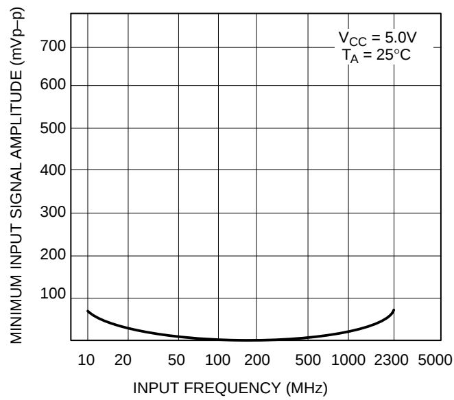
Figure 3. Input Signal Amplitude vs. Input Frequency
