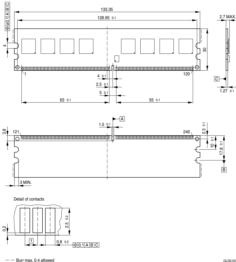
FIGURE 9 Package Outline L-DIM-240-8
