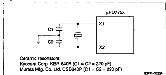
Figure 2. External Oscillator
