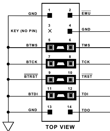
Figure 8. JTAG Target Board Connector with No Local Boundary Scan
