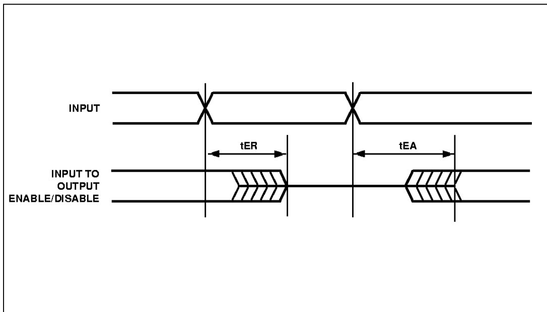
Figure 45. Input to Output Disable/Enable
