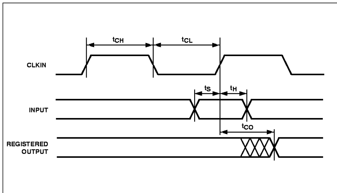
Figure 43. Synchronous Clock Mode Timing – ZPLD
