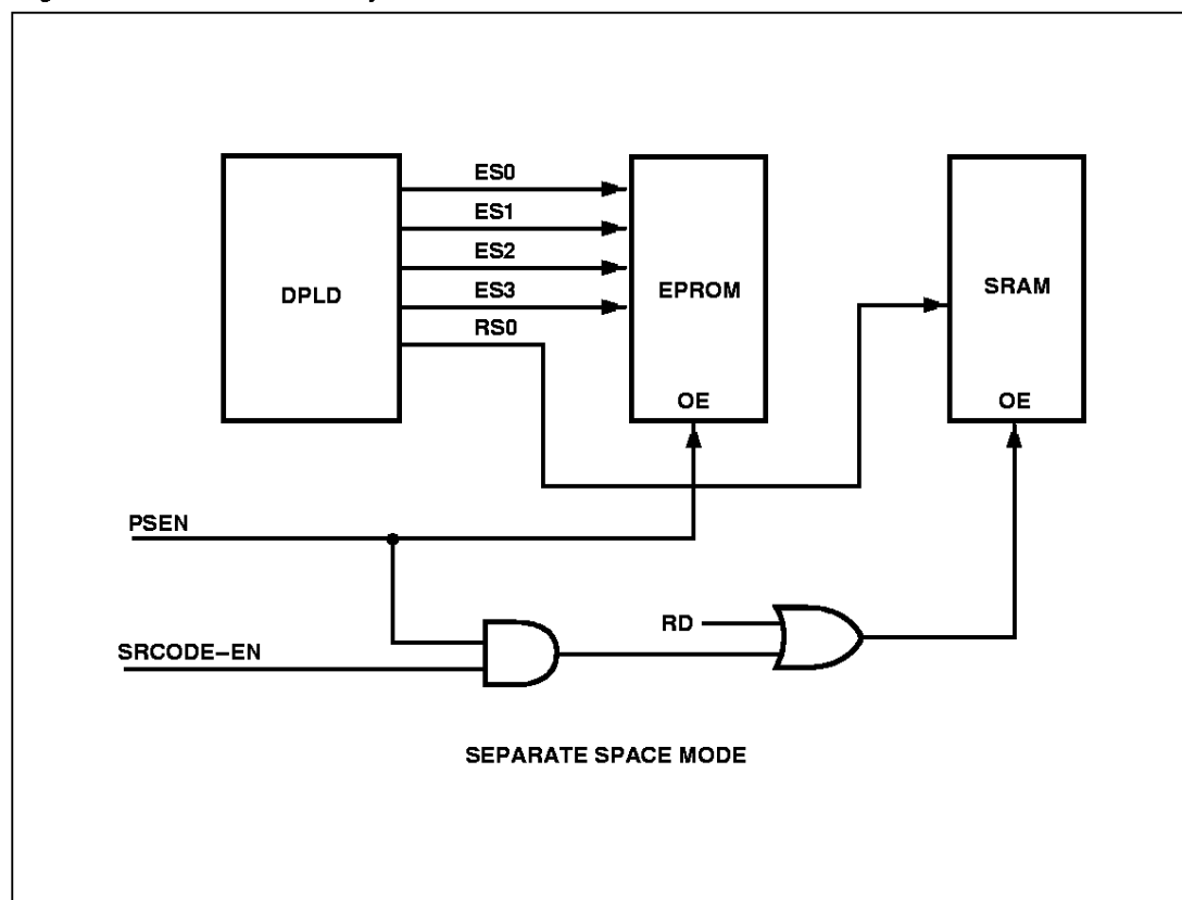
Figure 32a. 8031 Memory Modes
