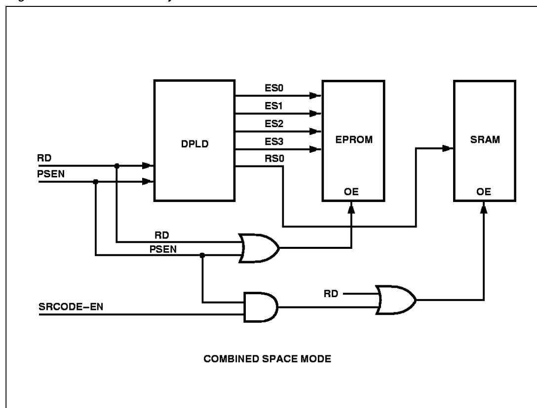
Figure 32b. 8031 Memory Modes
