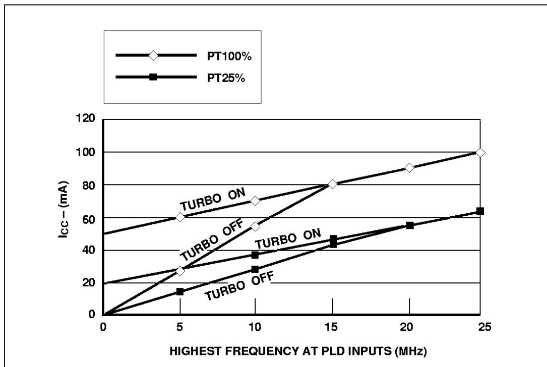
Figure 37b. ZPLD I_{CC} /Frequency Consumption
