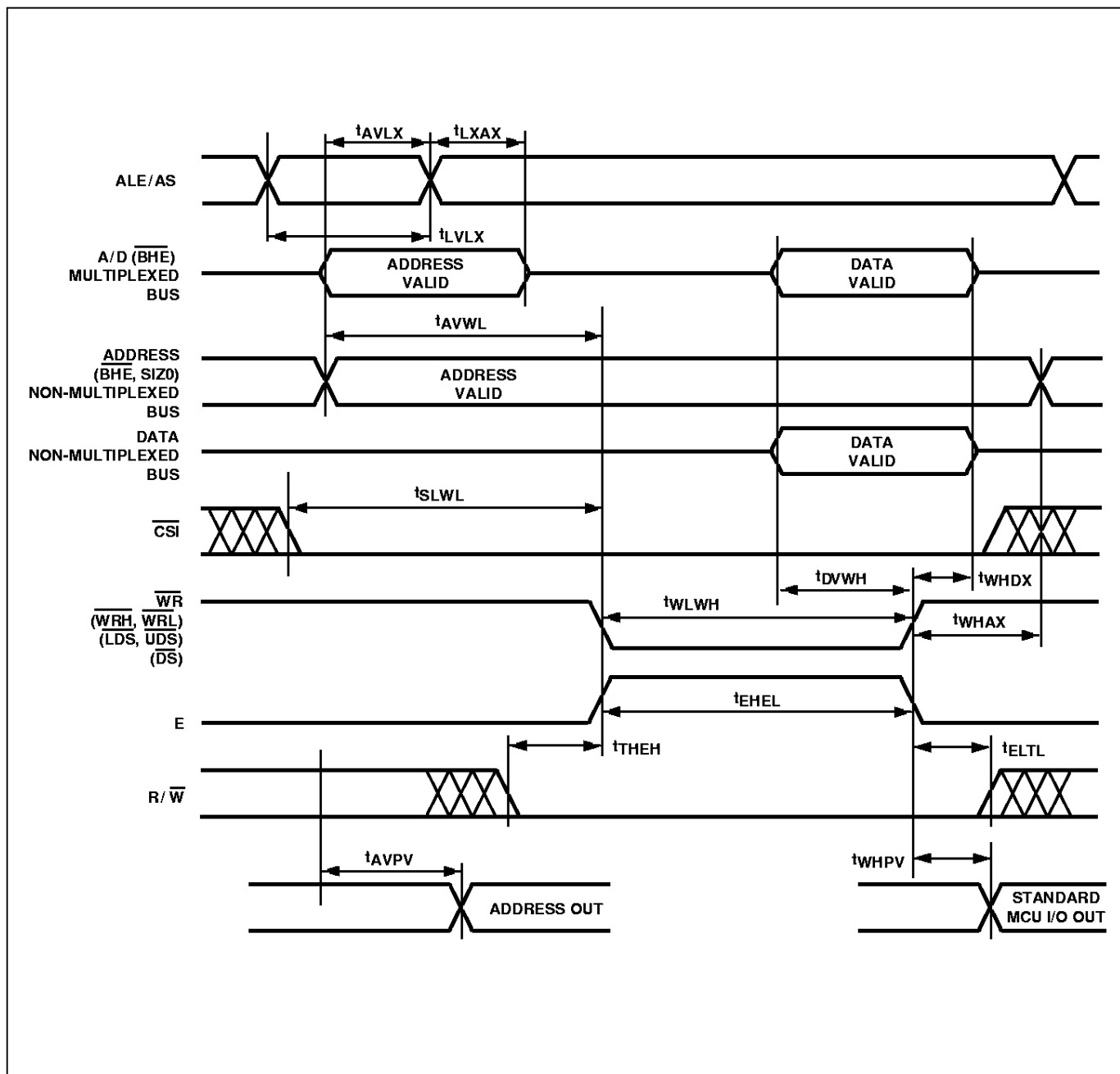
Figure 39. Write Timing
