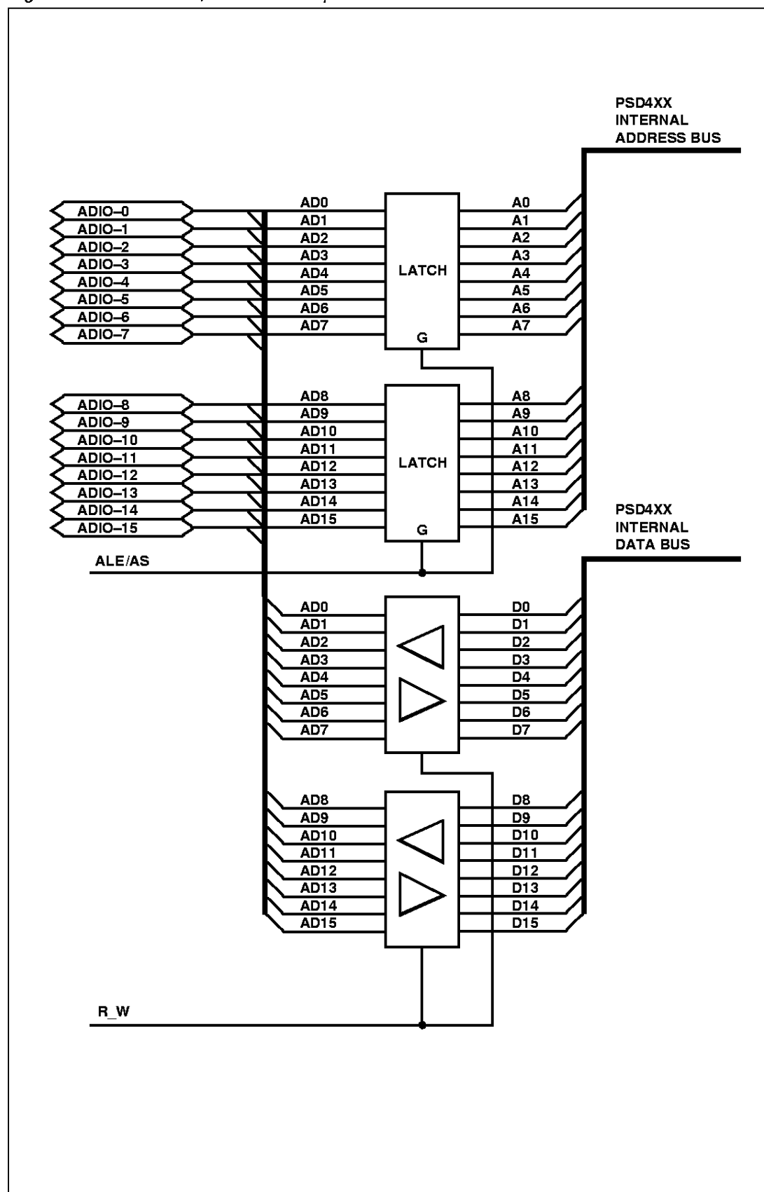
Figure 20. ADIO Port, 16-Bit Multiplexed Bus Interface
