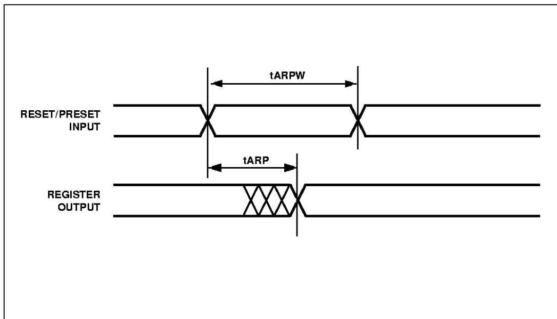
Figure 46. Asynchronous Reset/Preset
