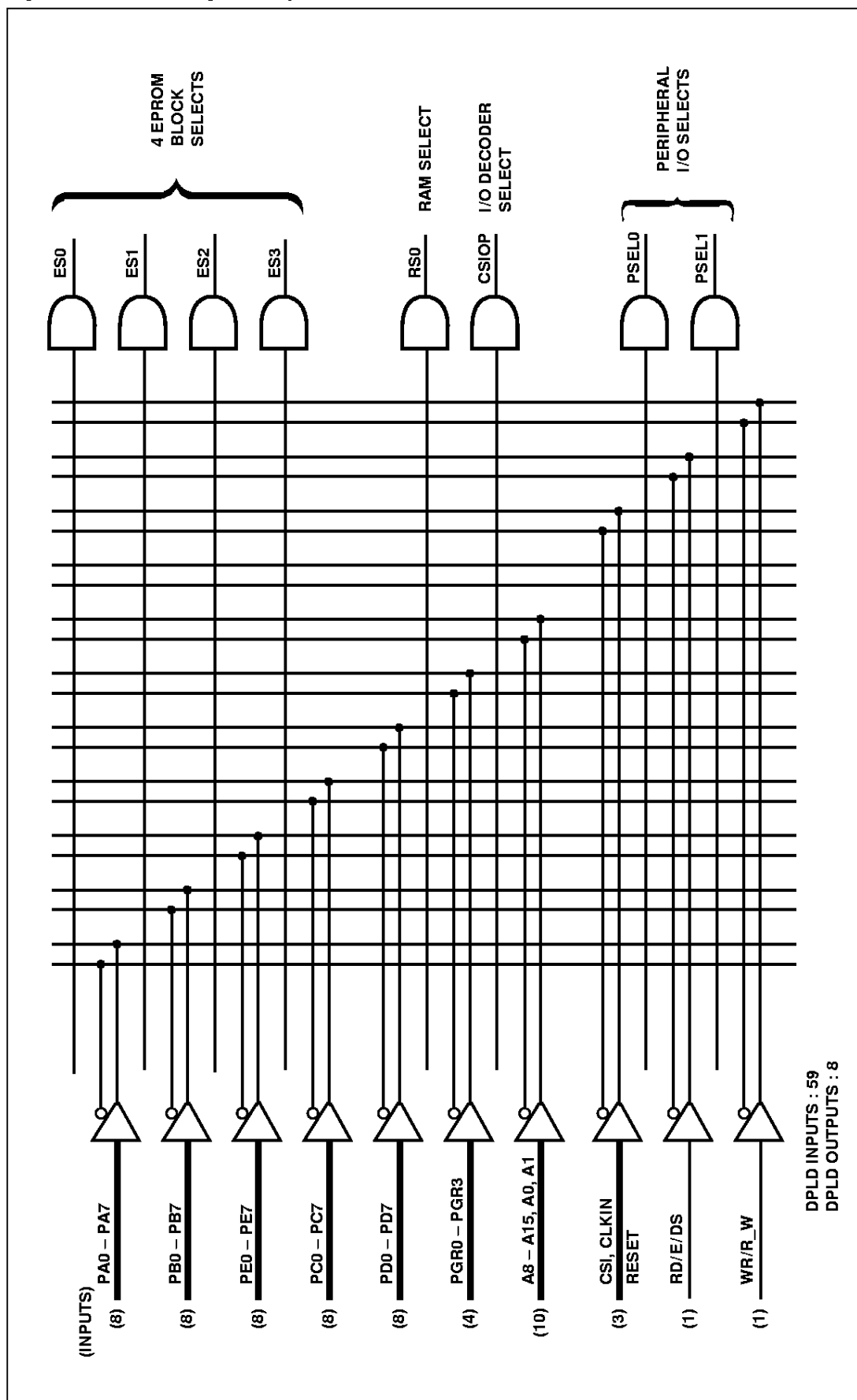
Figure 11. DPLD Logic Array
