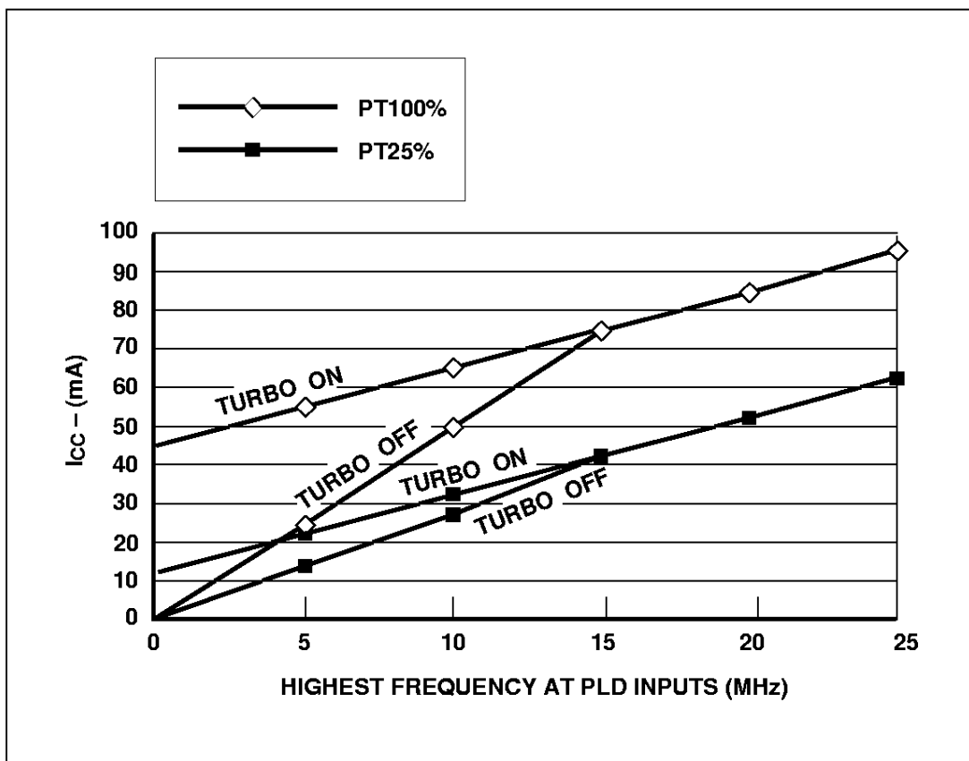
Figure 37a. ZPLD I_{CC} /Frequency Consumption (PSD4XXA1 Versions)
