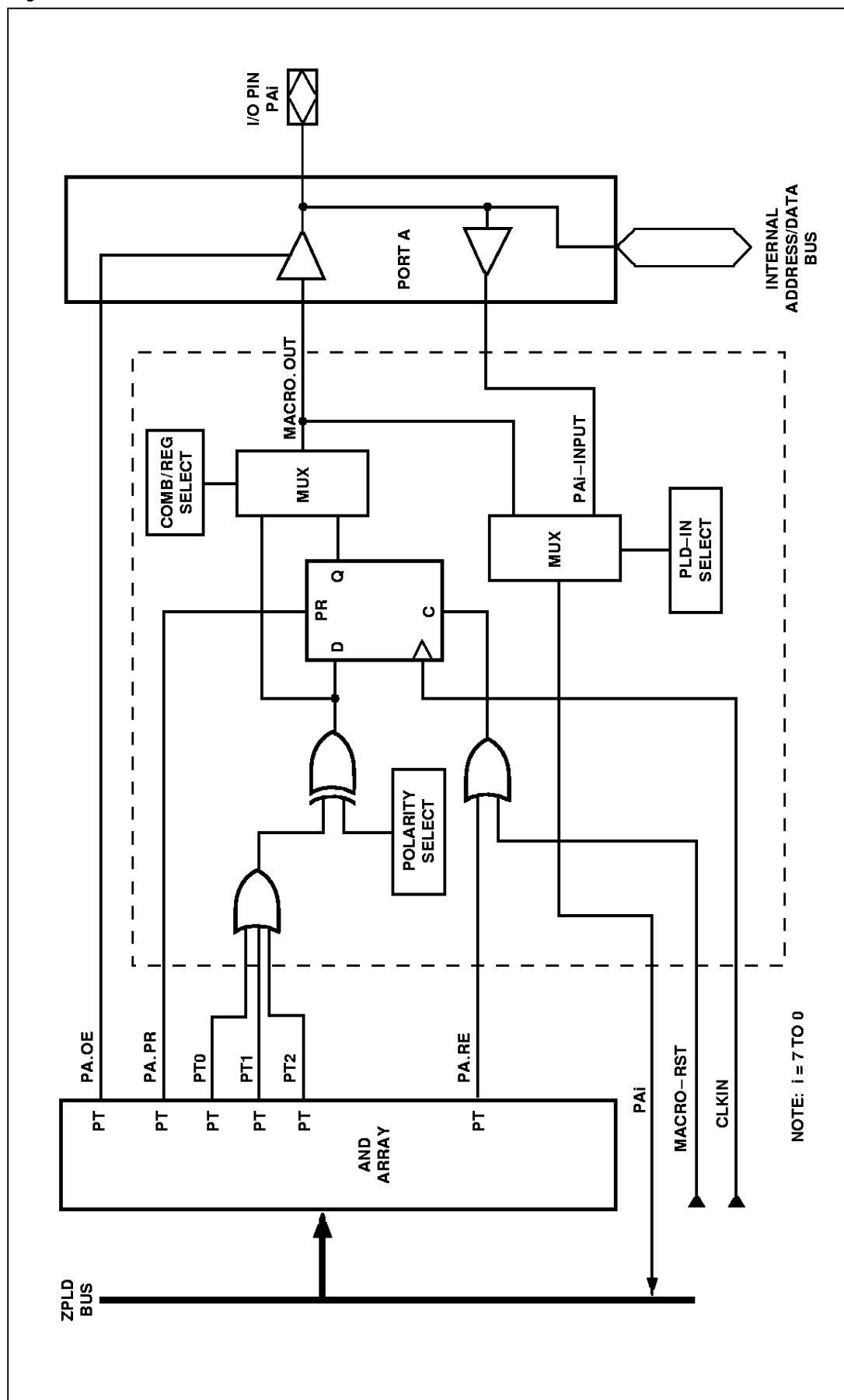
Figure 14. PSD4XXA2 PA Macrocell
