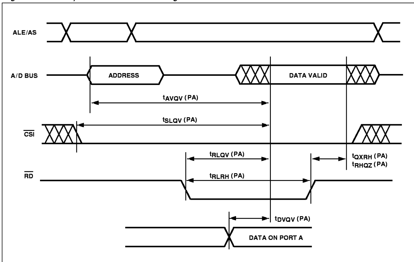
Figure 40. Peripheral I/O Read Timing
