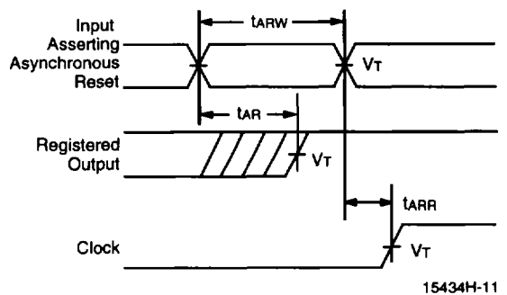
Asynchronous Reset
