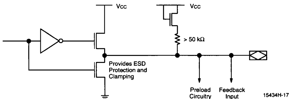
Typical Output
