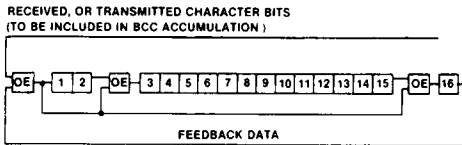
OPERATION OF BCC REGISTER FOR CRC-16 BCC ACCUMULATION (SIMPLIFIED)
