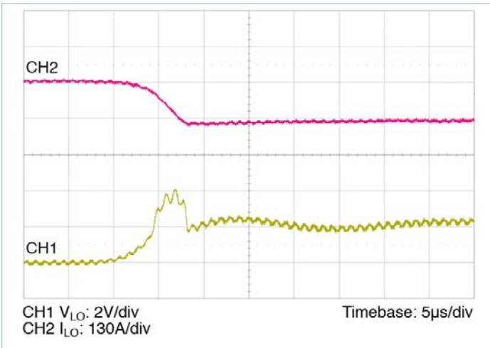
Figure 16 — 130A – 0A transient response: C_{HI\_IN\_EXT} = 300\mu\text{F} , no external C_{LO\_OUT\_EXT}
