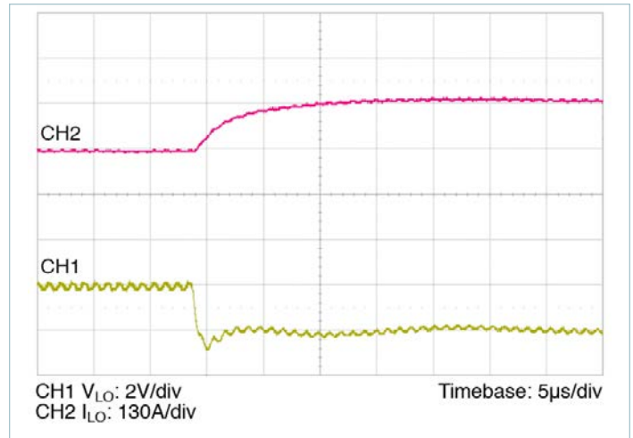
Figure 15 — 0A – 130A transient response: C_{HI\_IN\_EXT} = 300\mu\text{F} , no external C_{LO\_OUT\_EXT}
