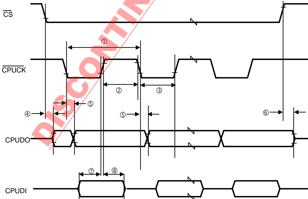
Figure 13 Serial CPU Interface Timing Chart
