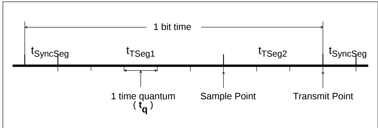
Figure 4: Bit Timing
