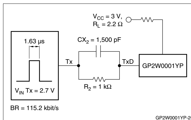
Figure 9. Recommended Emitter Circuit
