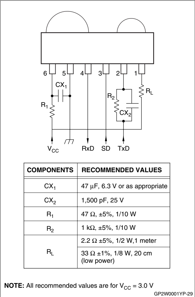
Figure 11. External Components
