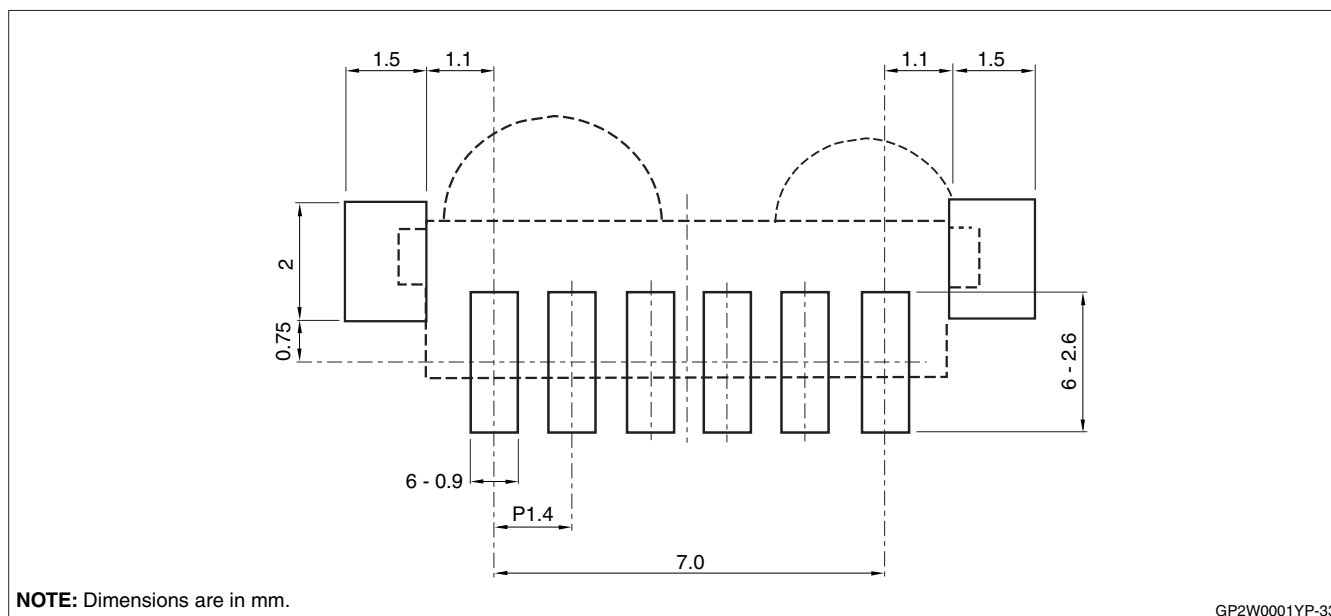
Figure 15. Recommended Footprint
