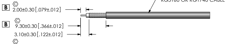
IN-PROCESS 1 STRIP AND TIN INNER CONDUCTOR
