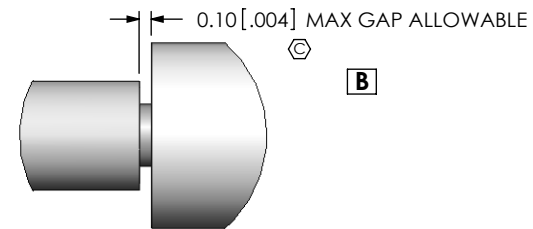
DETAIL 'B' SCALE 16:1
