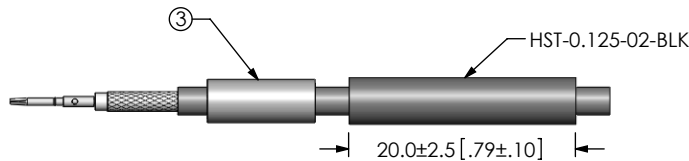
IN-PROCESS 3 ADD HEAT SHRINK TUBE AND FERRULE
