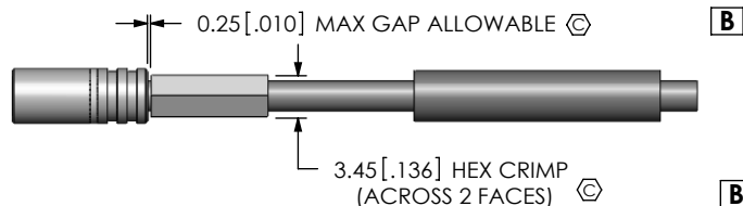
IN-PROCESS 6 CRIMP FERRULE (USE RF CRIMP HAND TOOL # CAT-HT-126667-21 OR EQUIVALENT) (USE .136" HEX DIE)
