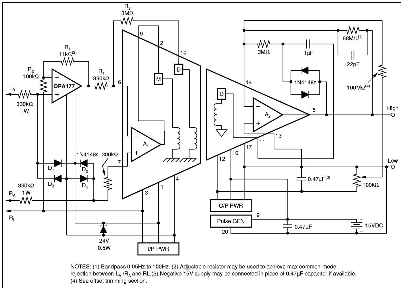
FIGURE 6. ECG Amplifier.
