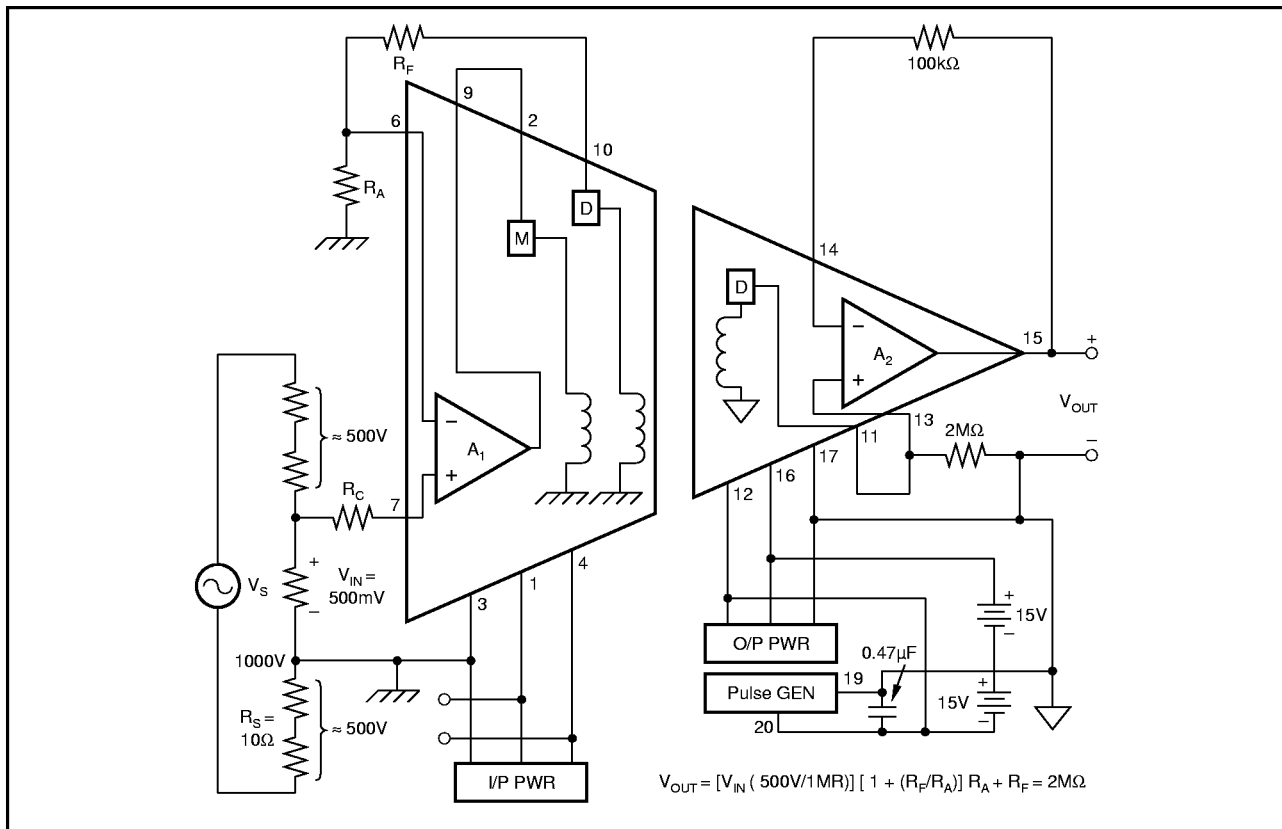
FIGURE 12. Series Source.
