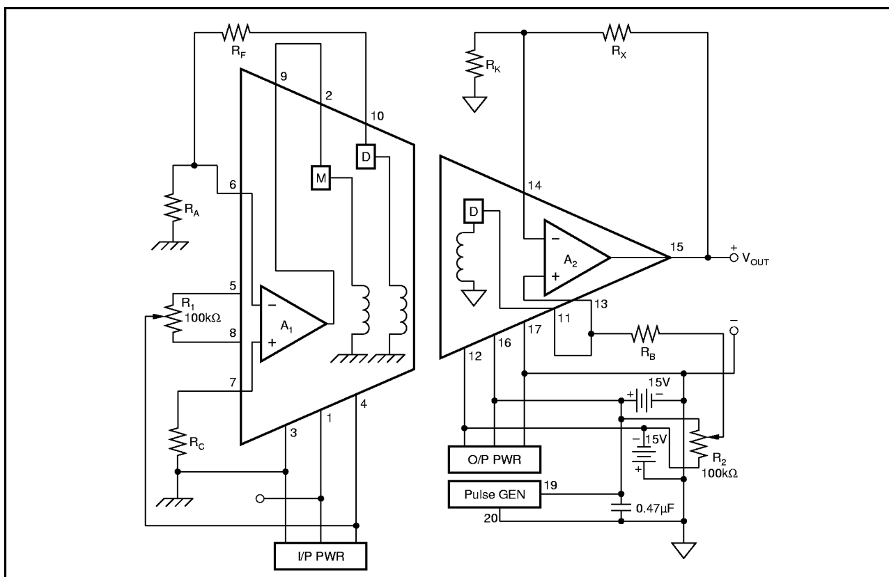
FIGURE 5. Optional Offset Voltage Trim.
