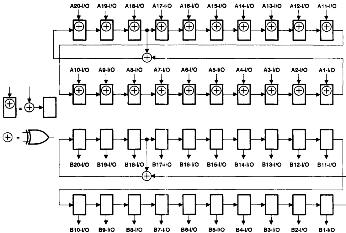
Figure 9. 20-Bit PSA/PRPG Configuration ( \overline{OEAB} = 0, OEBA = 1 )
