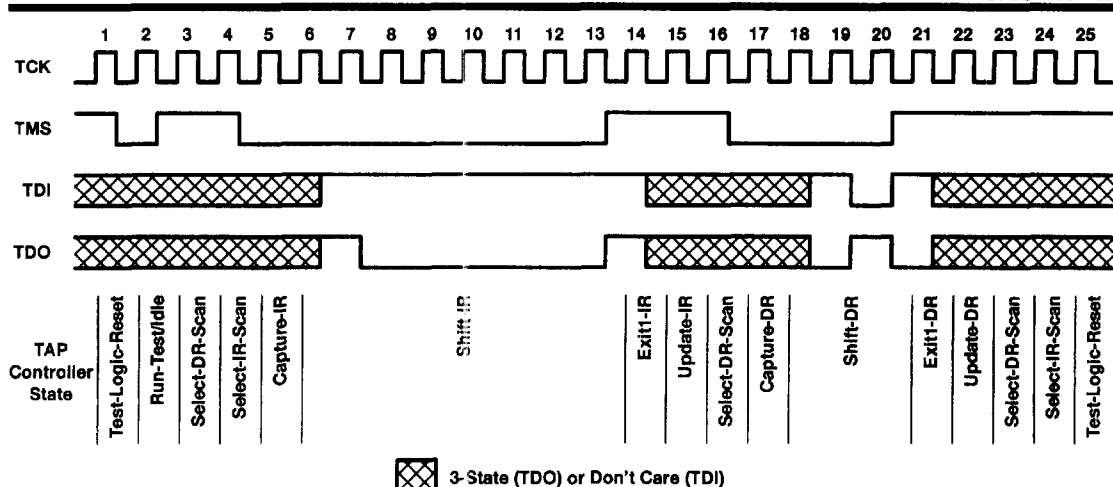
Figure 13. Timing Example
