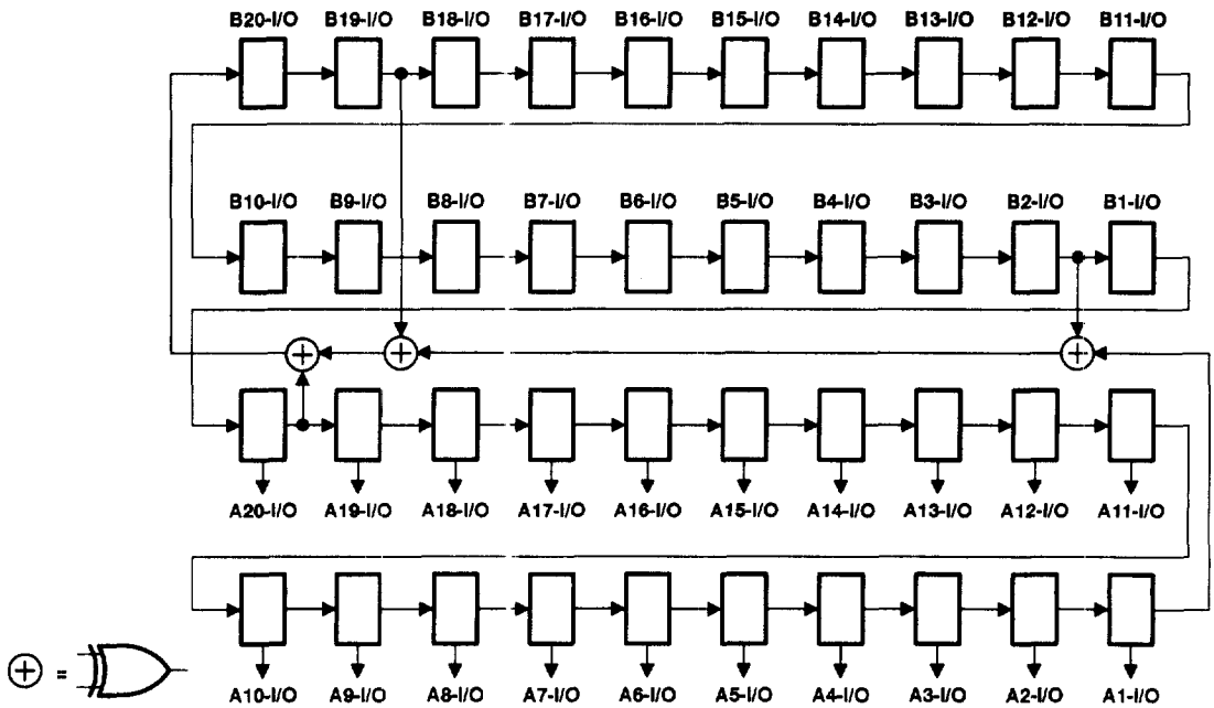
Figure 6. 40-Bit PRPG Configuration ( \overline{OEAB} = 1, \overline{OEBA} = 0 )
