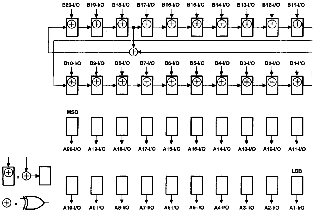
Figure 12. 20-Bit PSA/COUNT Configuration ( \overline{OEAB} = 1 , \overline{OEB\bar{A}} = 0 )
