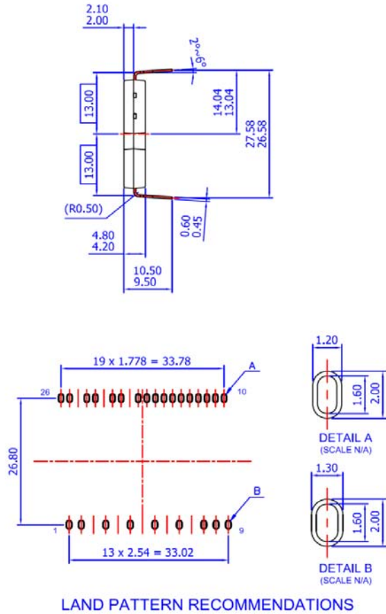
LAND PATTERN RECOMMENDATIONS
