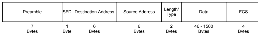
Figure 18-3. Ethernet Frame
