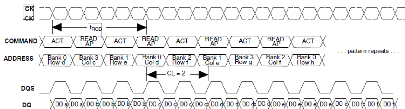
Timing waveform for IDD7 measurement at 100 MHz Ck operation
