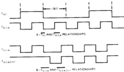
Figure 1. Transmit Data & Clock Relationships
