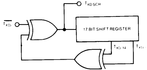
Figure 2. 17 Bit Pseudo Random Scrambler
