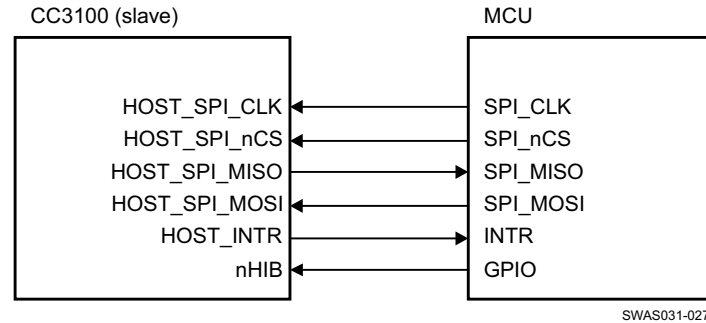
Figure 4-15. SPI Host Interface
