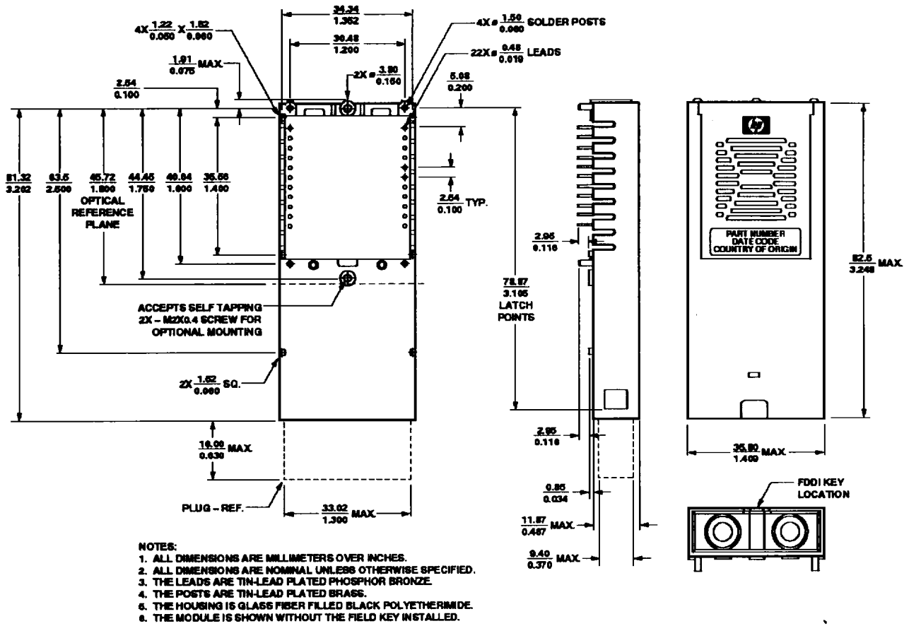
Figure 2(a). HFBR-5111 Outline Drawing.
