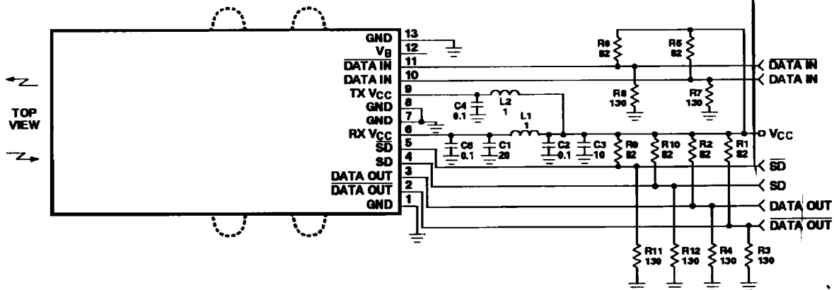
(a) HFBR-5111
