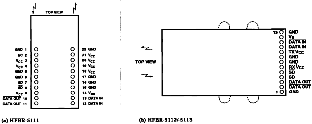
Figure 3. Pin Assignments.
