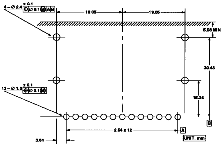
(b) HFBR-5112
