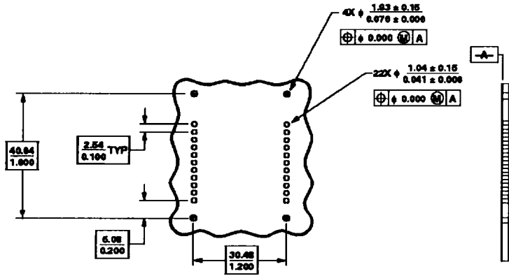
(a) HFBR-5111
