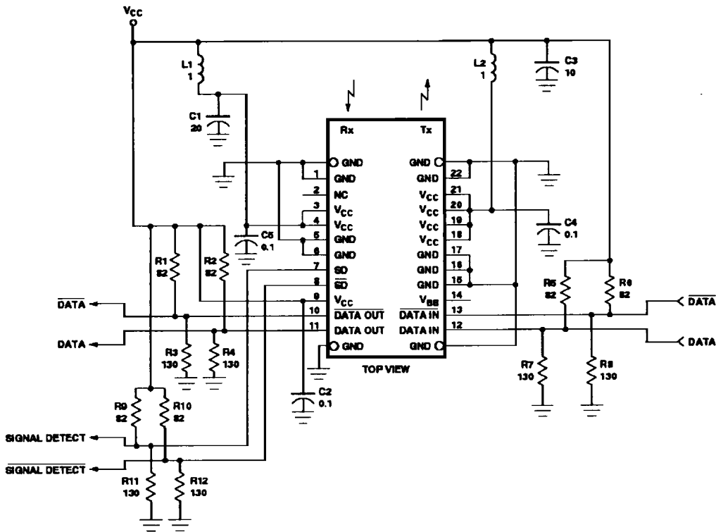
(a) HFBR-5111
