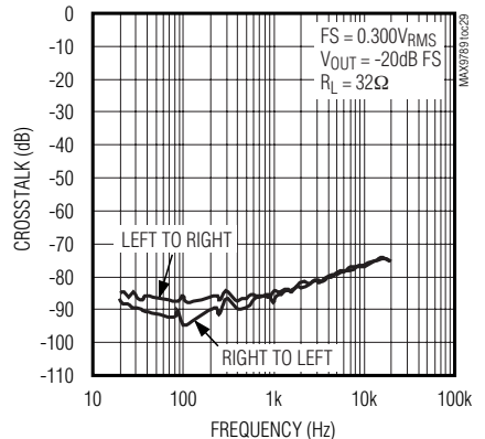
CROSSTALK vs. FREQUENCY (HEADPHONE MODE)
