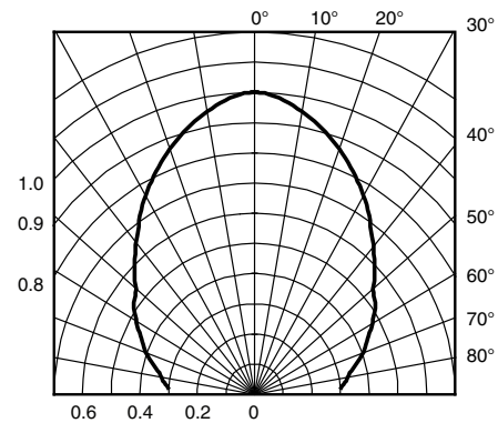
Fig. 13 - Vertical Directivity
