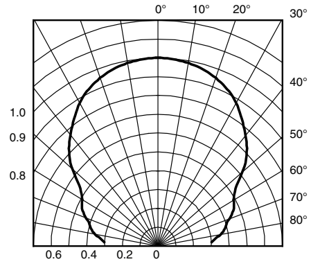
Fig. 12 - Horizontal Directivity
