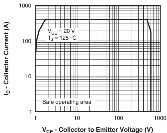
Fig. 12 - Turn-Off SOA
