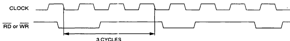
Figure 7 : Typical I/O Timing
