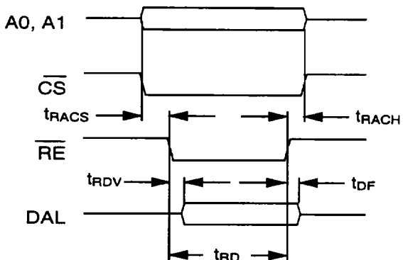
Figure 5 : Read Timing
