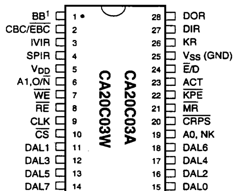
a) 28-pin PDIP
