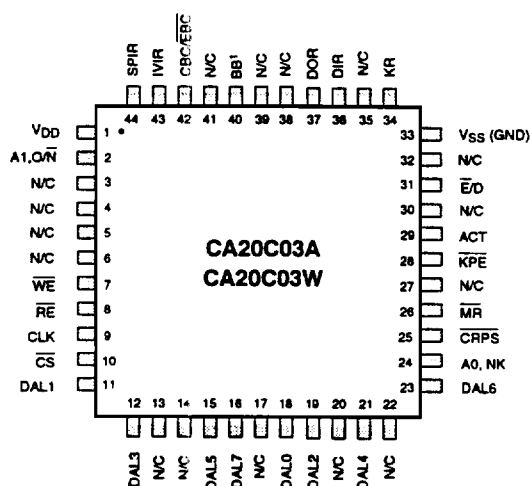
c) 44-lead TQFP
