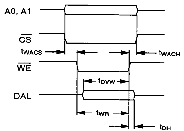
Figure 6 : Write Timing
