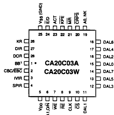
b) 28-lead PLCC
