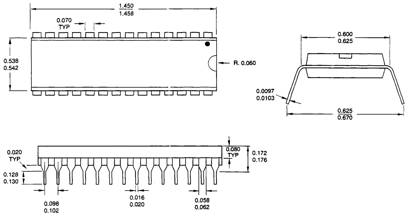
Figure 15 : 28-Pin PDIP Packaging
