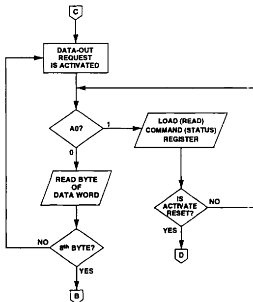
Figure 13 : Activating DOR Output Procedure (ECB Mode Only)
