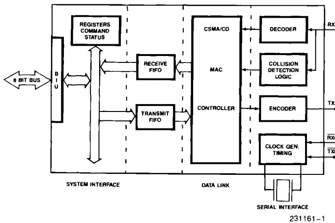
Figure 1. 82588 Block Diagram
