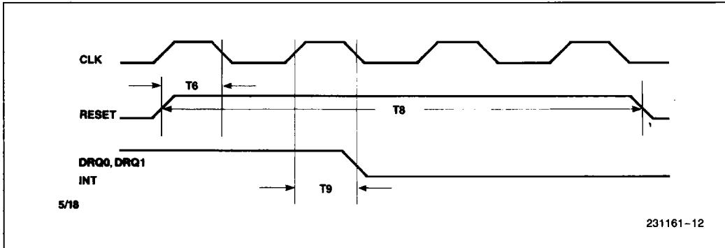
Reset Timing
