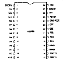
231161-2 Figure 2. 82588 Pin Configuration (DIP)
