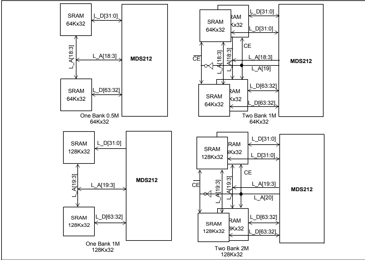
Figure 3 - Frame Buffer Memory Configuration
