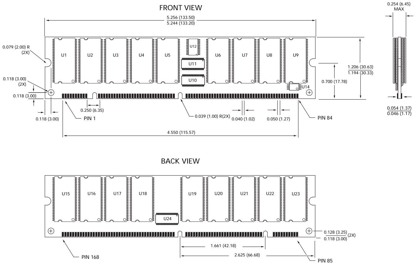
Figure 12: 168-Pin DIMM Dimensions – Low-Profile
