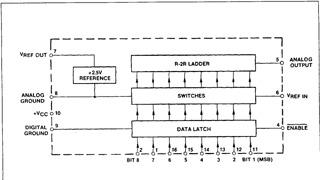
Fig.2 System diagram
