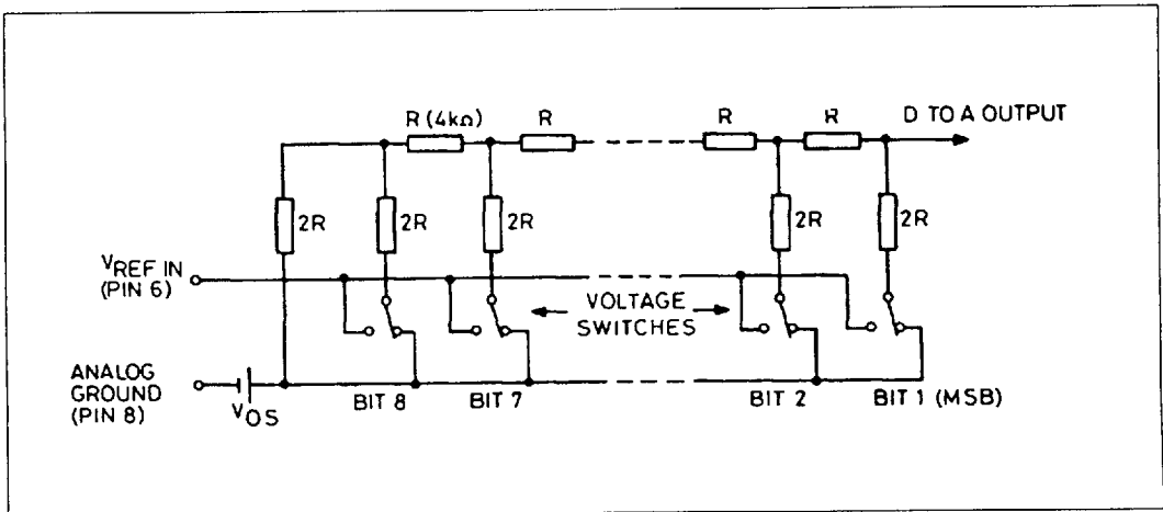
Fig.3 The R-2R ladder network
