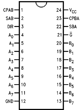
Pin Assignment for DIP and Flatpack
