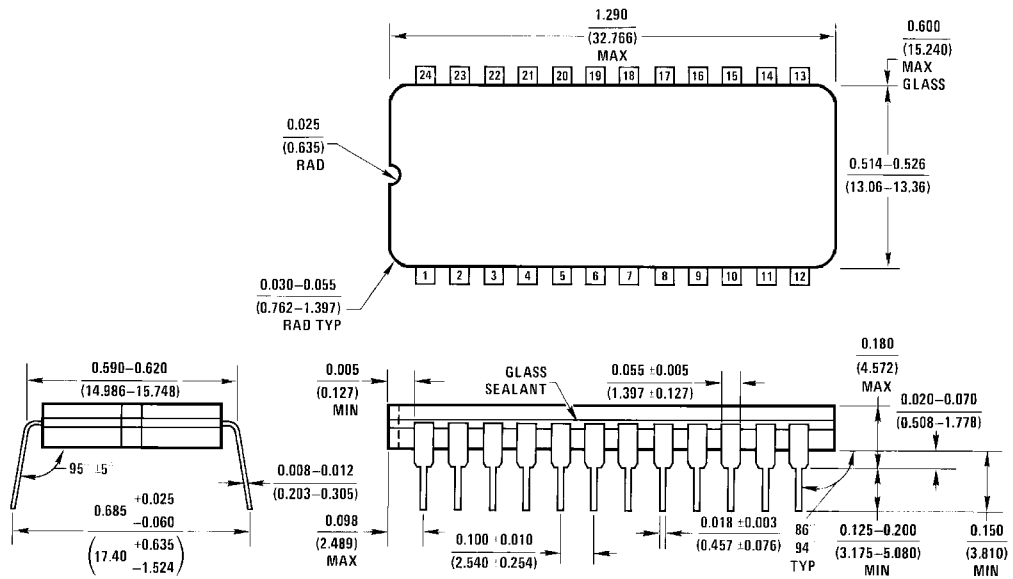
24-Lead Ceramic Dual-In-Line Package Number J24A
