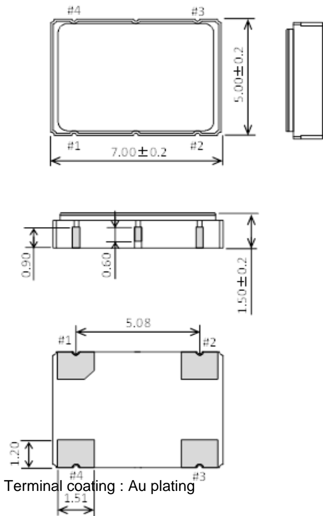
[ 8 ] Outline Drawing unit: mm
