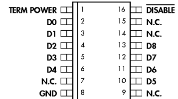
DW PACKAGE (Top View)
