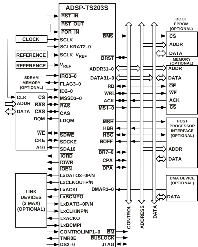
Figure 2. ADSP-TS203S Single-Processor System With External SDRAM
