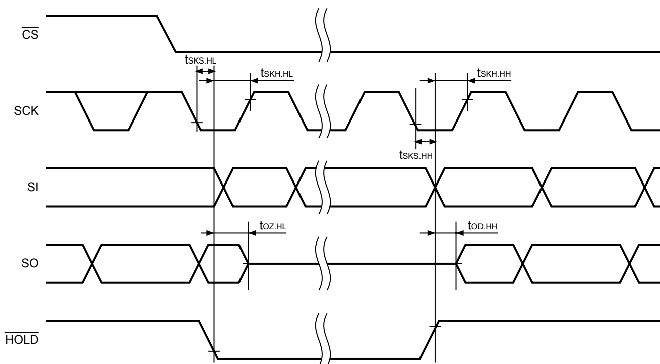
Figure 4 Hold Timing
