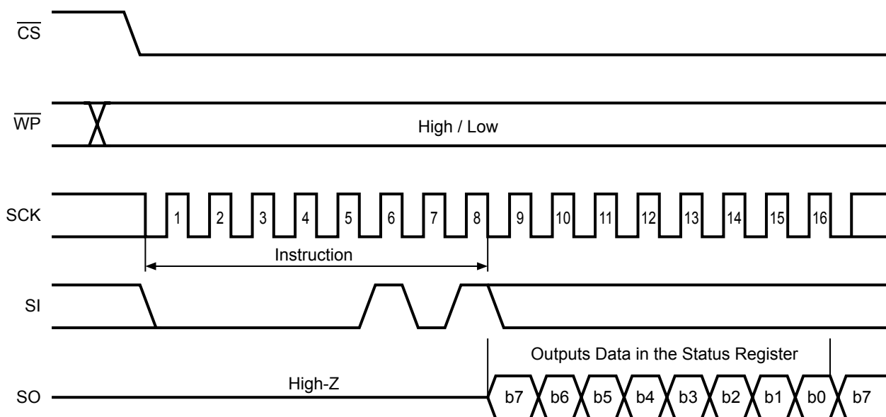
Figure 12 RDSR Operation
