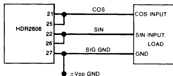
FIGURE 12 Output Connections For Short Cable Length
