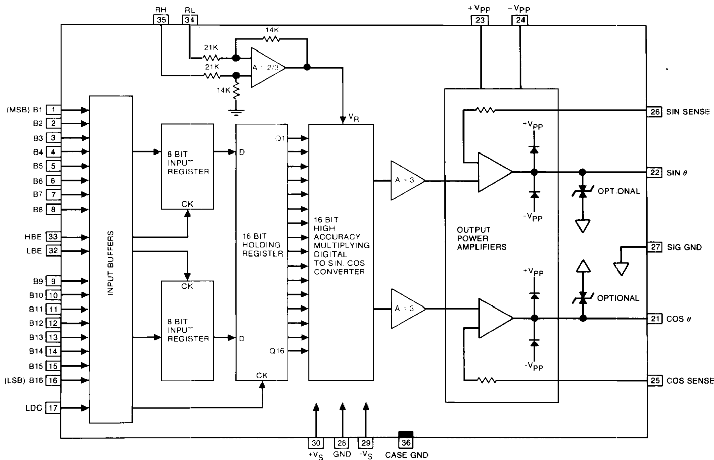
FIGURE 1 2606 Block Diagram
