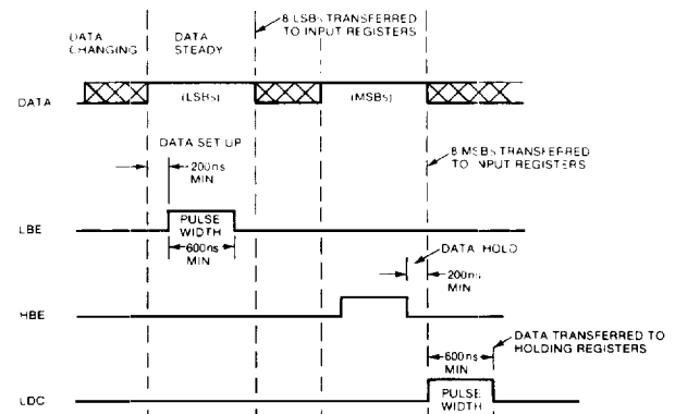
FIGURE 5 Two-Byte Loading
