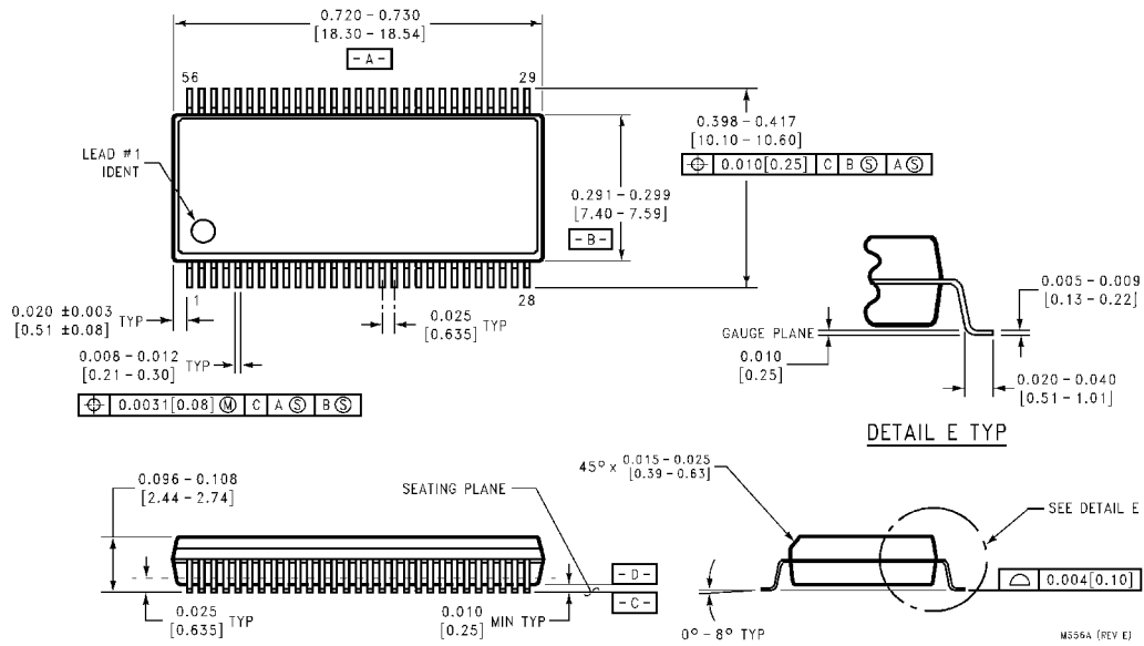
56-Lead SSOP (0.300" Wide) (SS) Order Number SCAN18540TSSC or SCAN18540TSSCX Package Number MS56A
