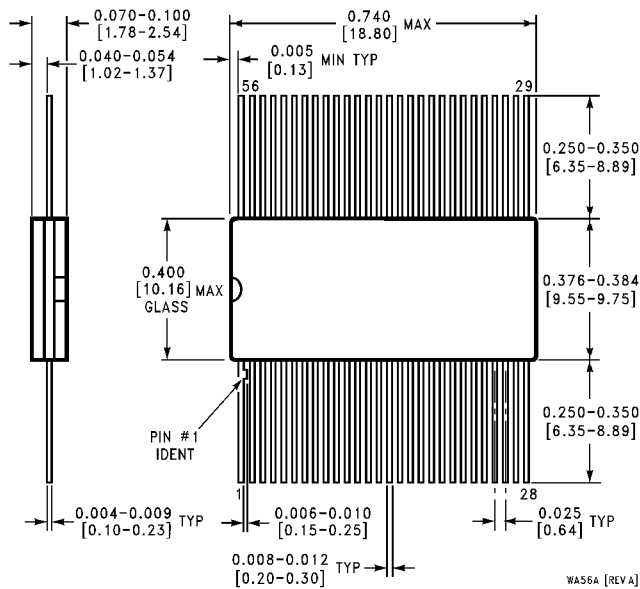
56-Lead Ceramic Flatpak (F) Order Number SCAN18540TFMQB Package Number WA56A
