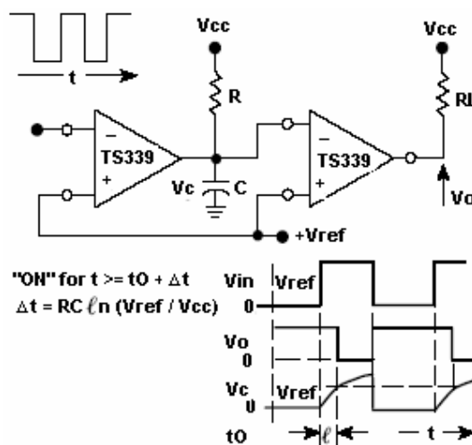
Figure 7. time delay generator
