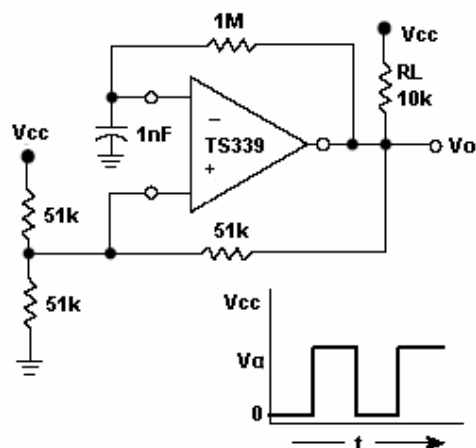
Figure 6. free-running square-wave oscillator
