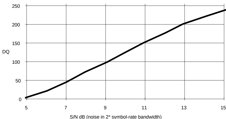
Figure 14 Typical Data Quality Reading vs S/N
