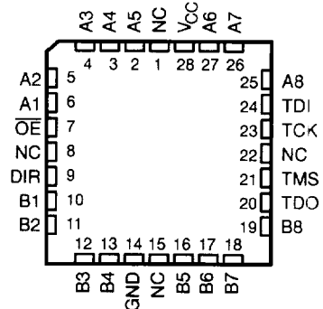
SN54BCT8245A ... FK PACKAGE (TOP VIEW)
