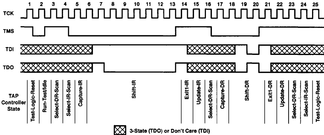
Figure 8. Timing Example
