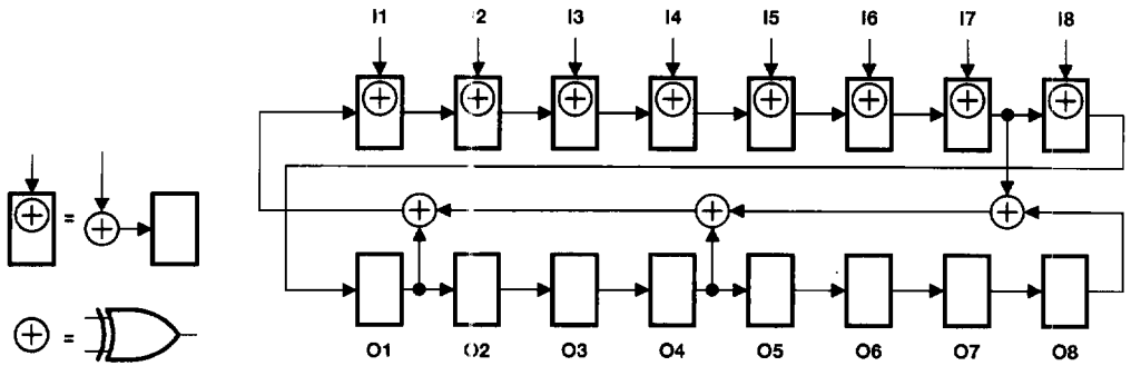
Figure 6. 16-Bit PSA Configuration
