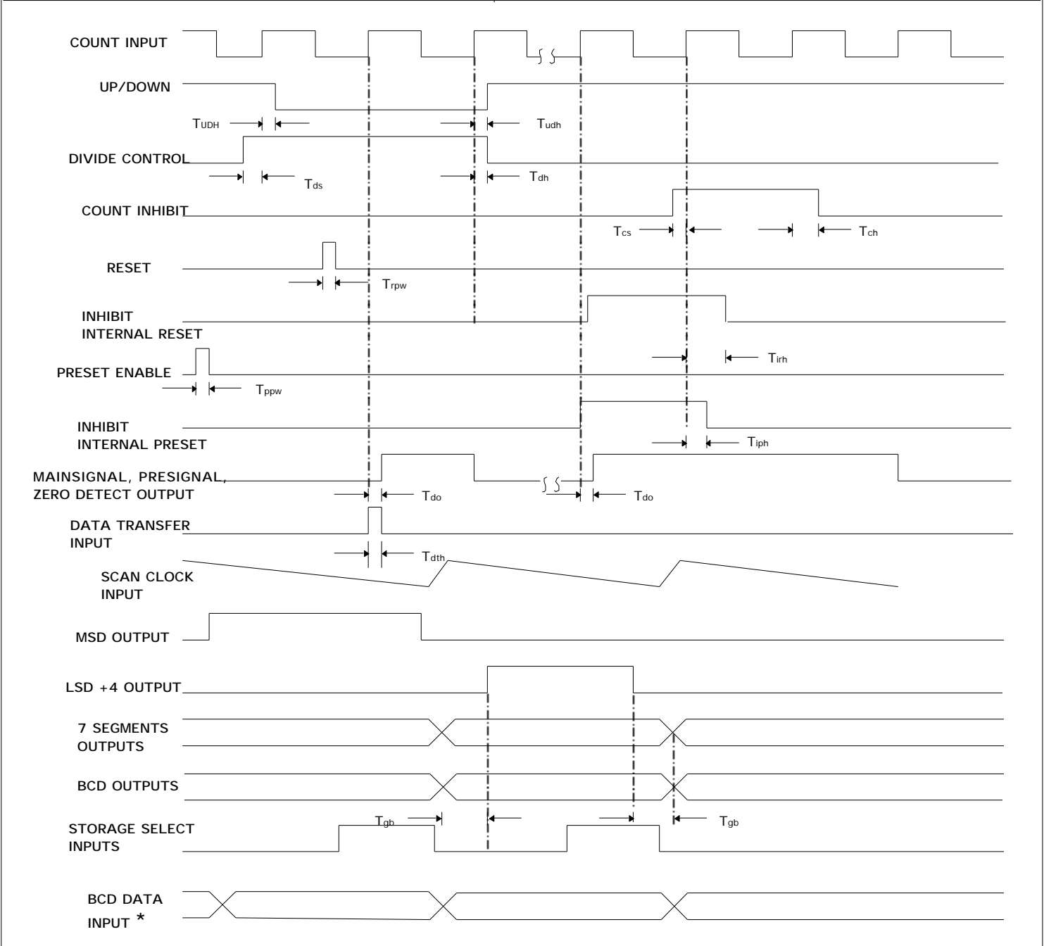
FIGURE 4. TIMING DIAGRAM
