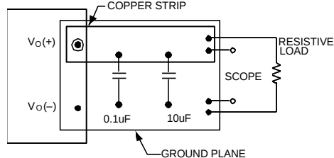
Figure 13. Input Reflected Ripple Current Test Setup.
