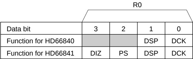
Figure 20 Control Register 1
