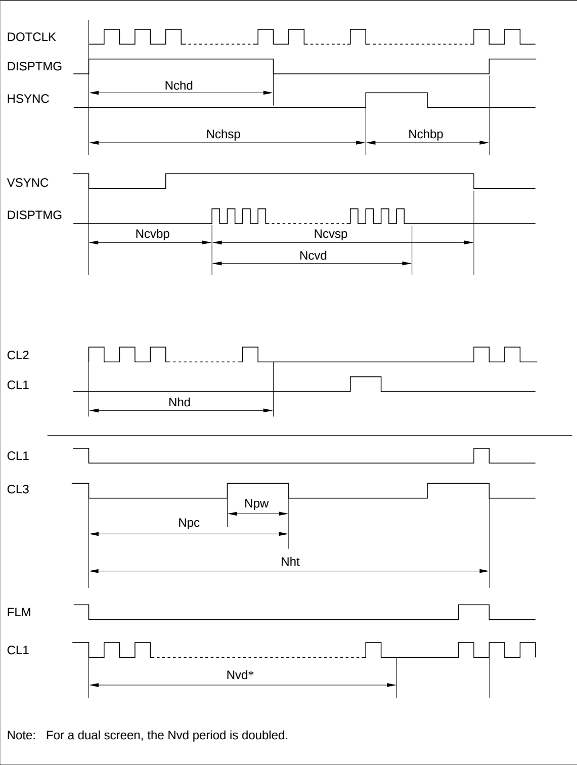
Figure 33 Symbol Definitions
