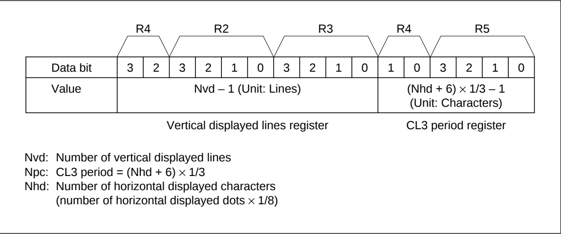
Figure 23 Vertical Displayed Lines Register and CL3 Period Register
