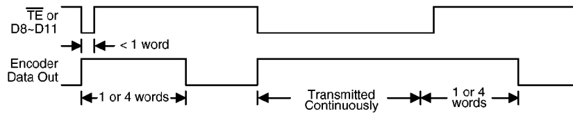
Transmission timing
