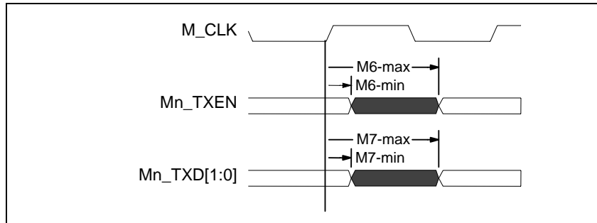
Figure 16 - AC Characteristics – Reduced Media Independent Interface
