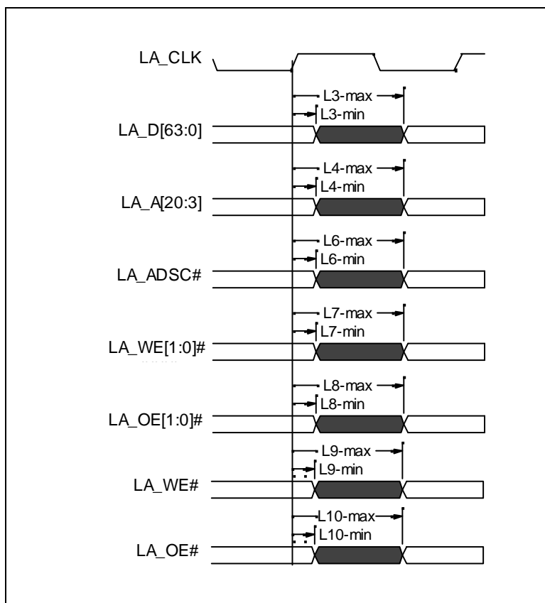
Figure 15 - Local Memory Interface - Output Valid Delay Timing
