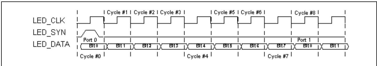
Figure 4 - Timing Diagram of LED Interface
