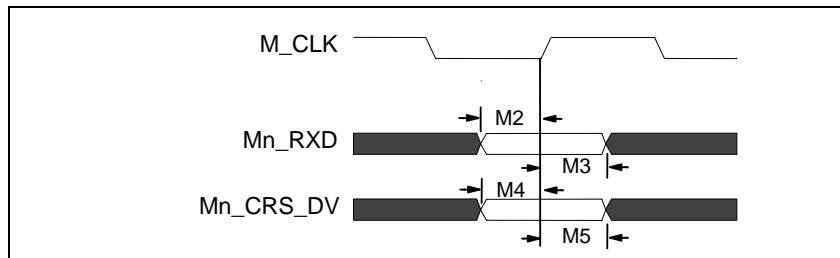
Figure 17 - AC Characteristics – Reduced Media Independent Interface
