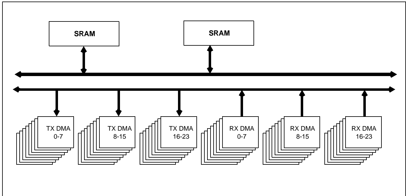
Figure 6 - SRAM Interface Block Diagram (DMAs for 10/100 Ports Only)
