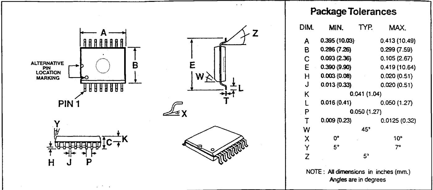
Figure 10: 16-pin SOIC Mechanical Outline: order as part no. CMX631AD4
