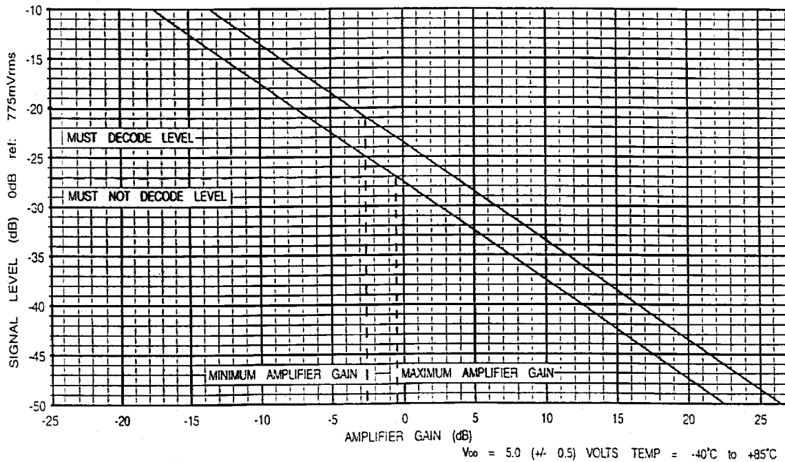
Figure 5: Input Gain Calculation Graph for V_{DD} = 5.0V
