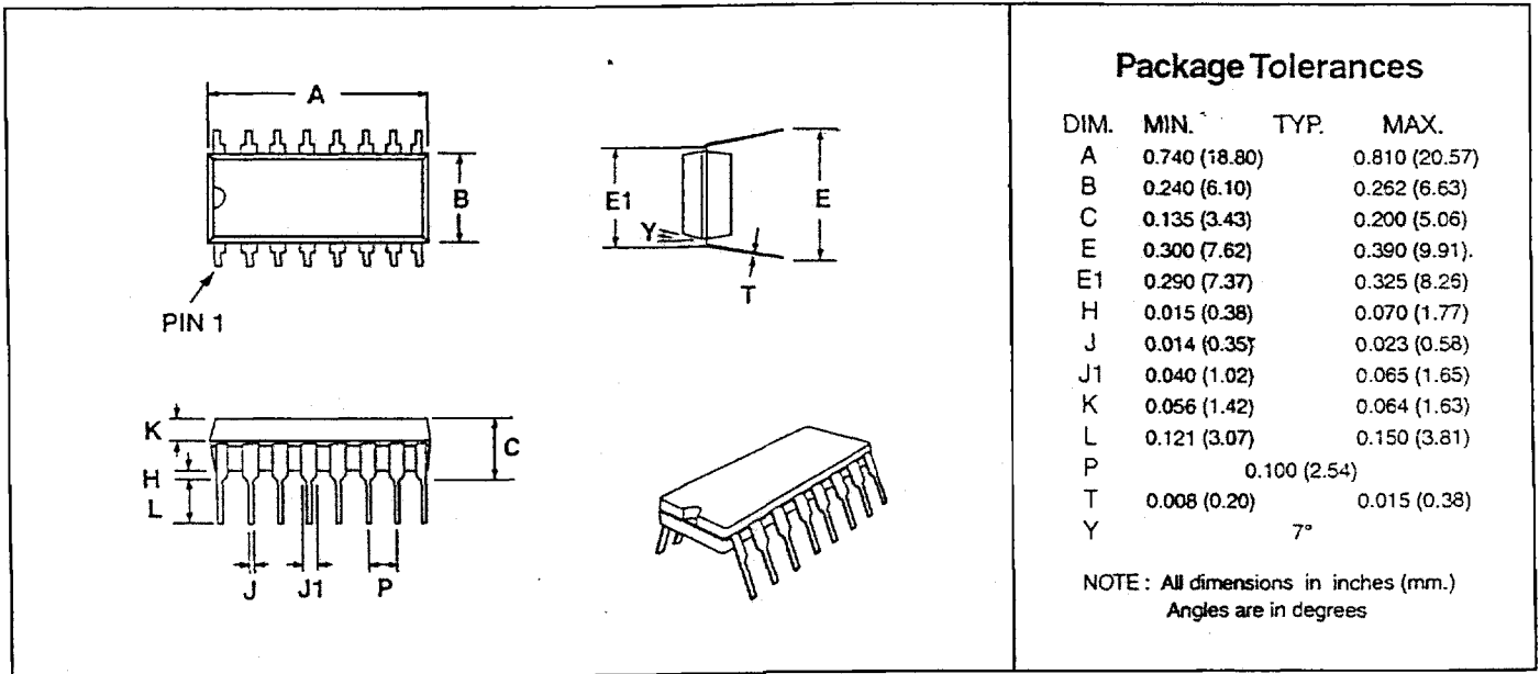
Figure 11: 16-pin PDIP Mechanical Outline: order as part no. CMX631AP3
