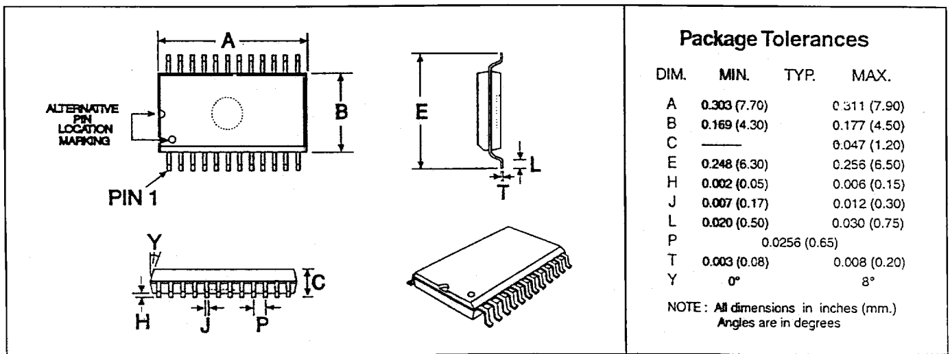
Figure 8: 24-pin TSSOP Mechanical Outline: order as part no. CMX631AE2
