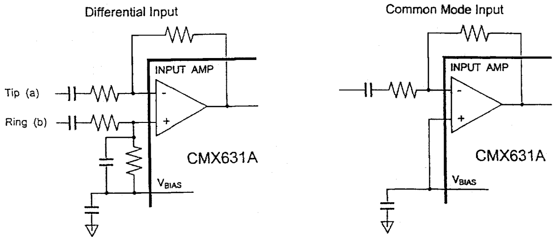
Figure 7: Input Configurations
