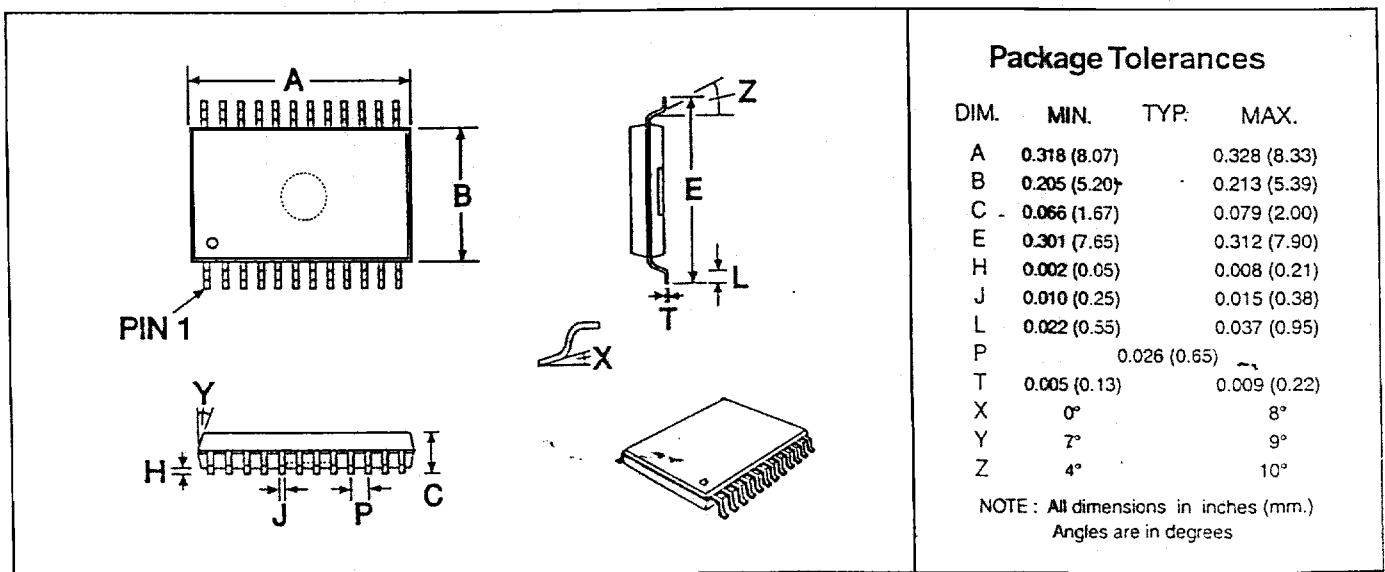
Figure 9: 24-pin SSOP Mechanical Outline: order as part no. CMX631AD5
