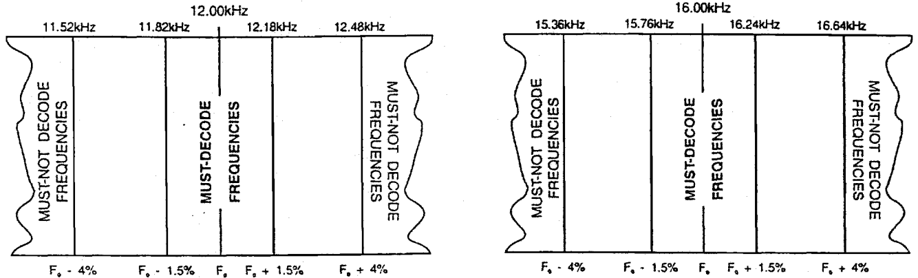
Figure 6: 'Must'/'Must Not' Decode Frequencies
