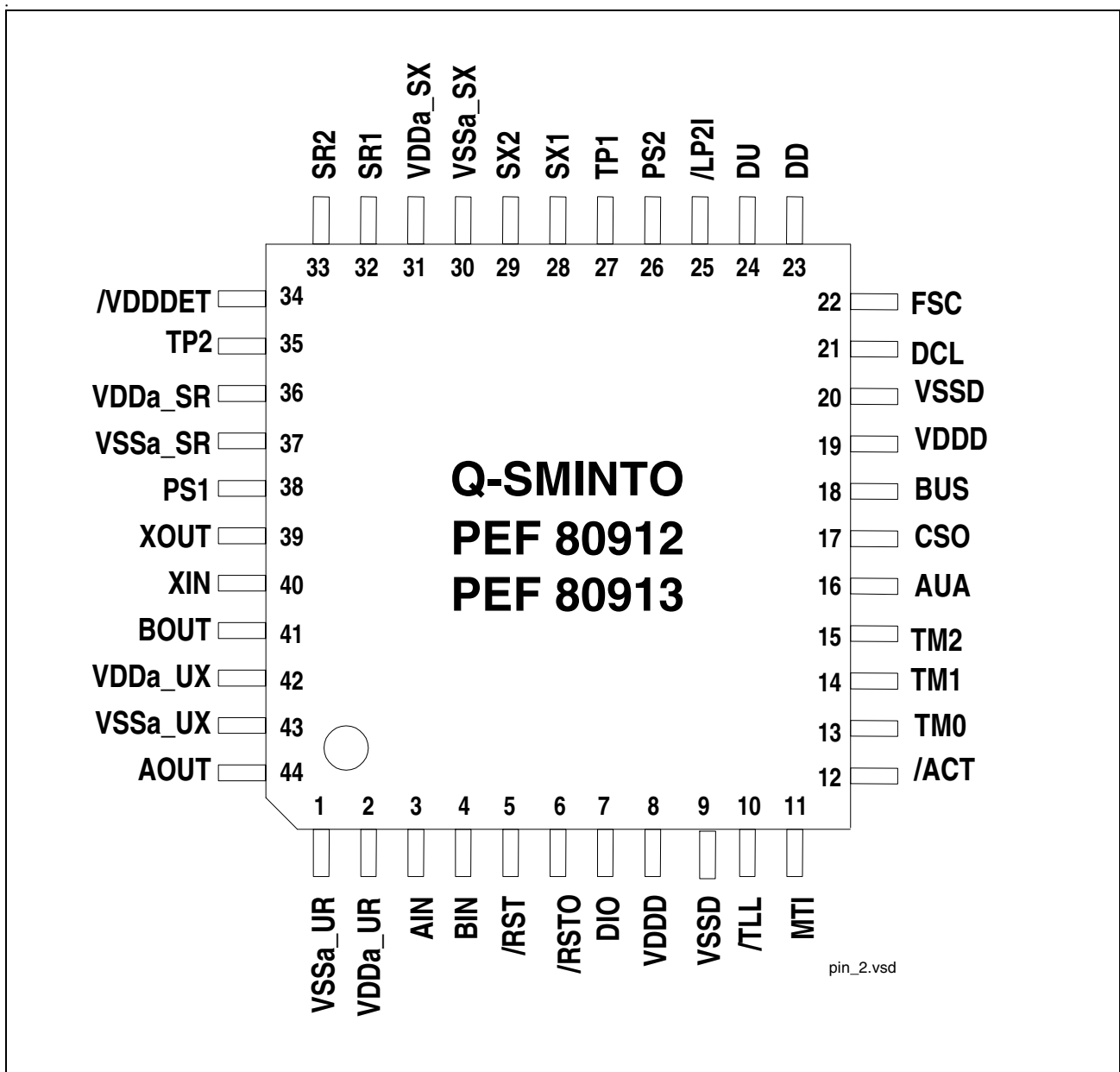
Figure 1 Pin Configuration
