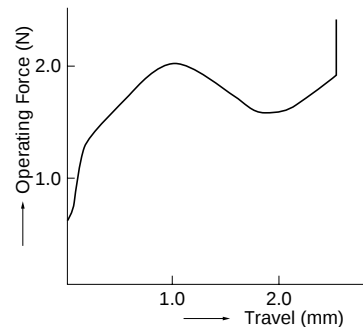
F-S Characteristics
