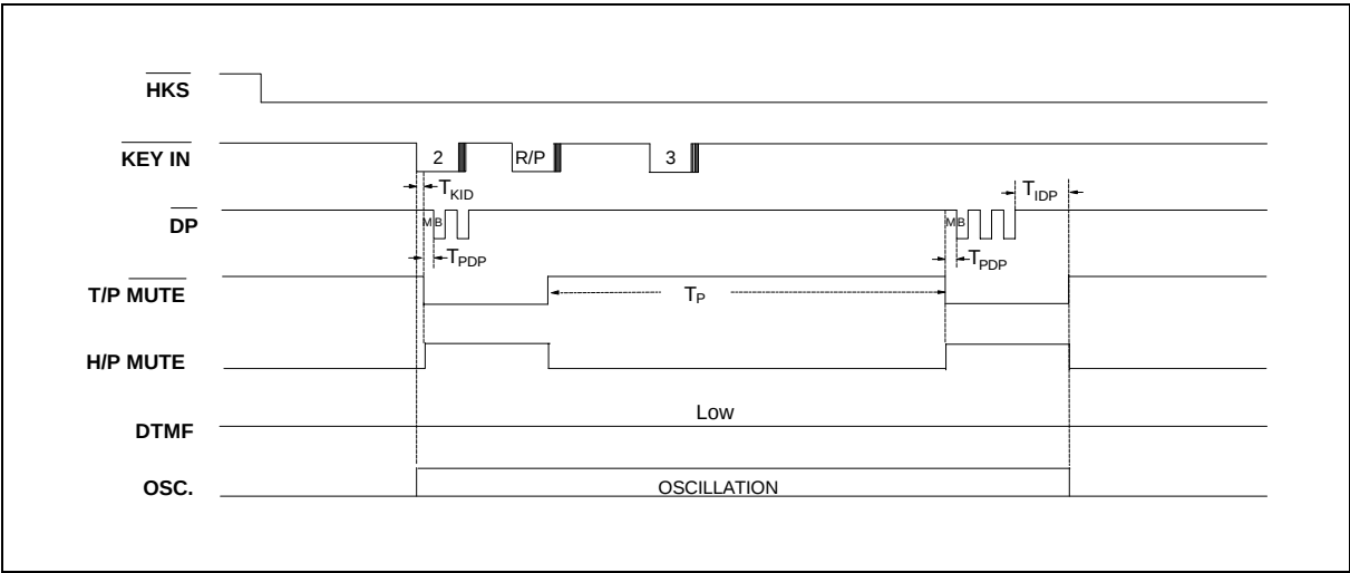
Figure 4. Pause Function Timing Diagram
