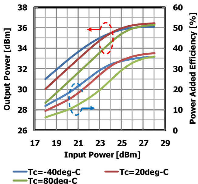
Input Power vs. Output Power, Power Added Efficiency by Temperature V_{DS}=10V @7.9GHz
