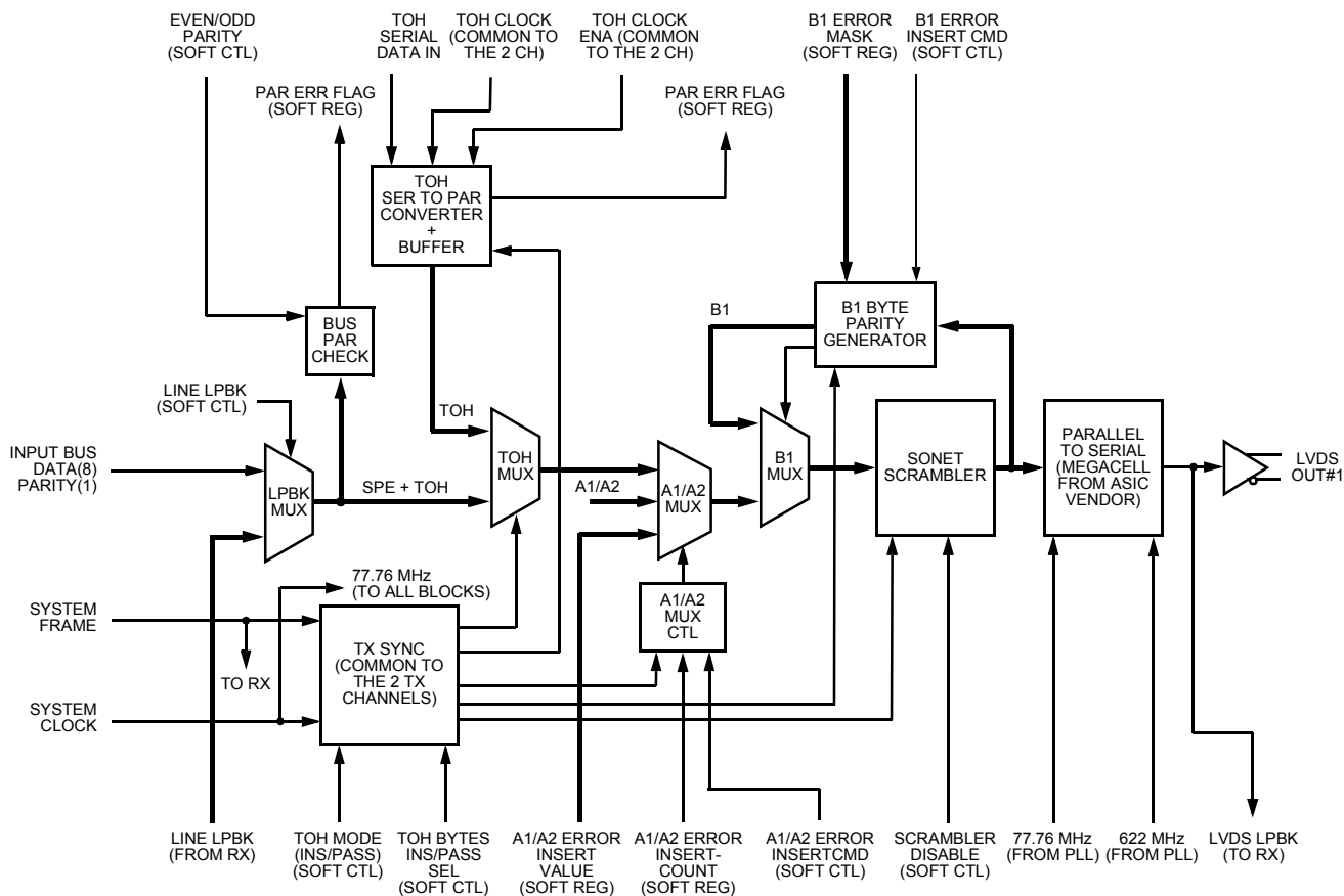
Figure 7. Transmitter Block
