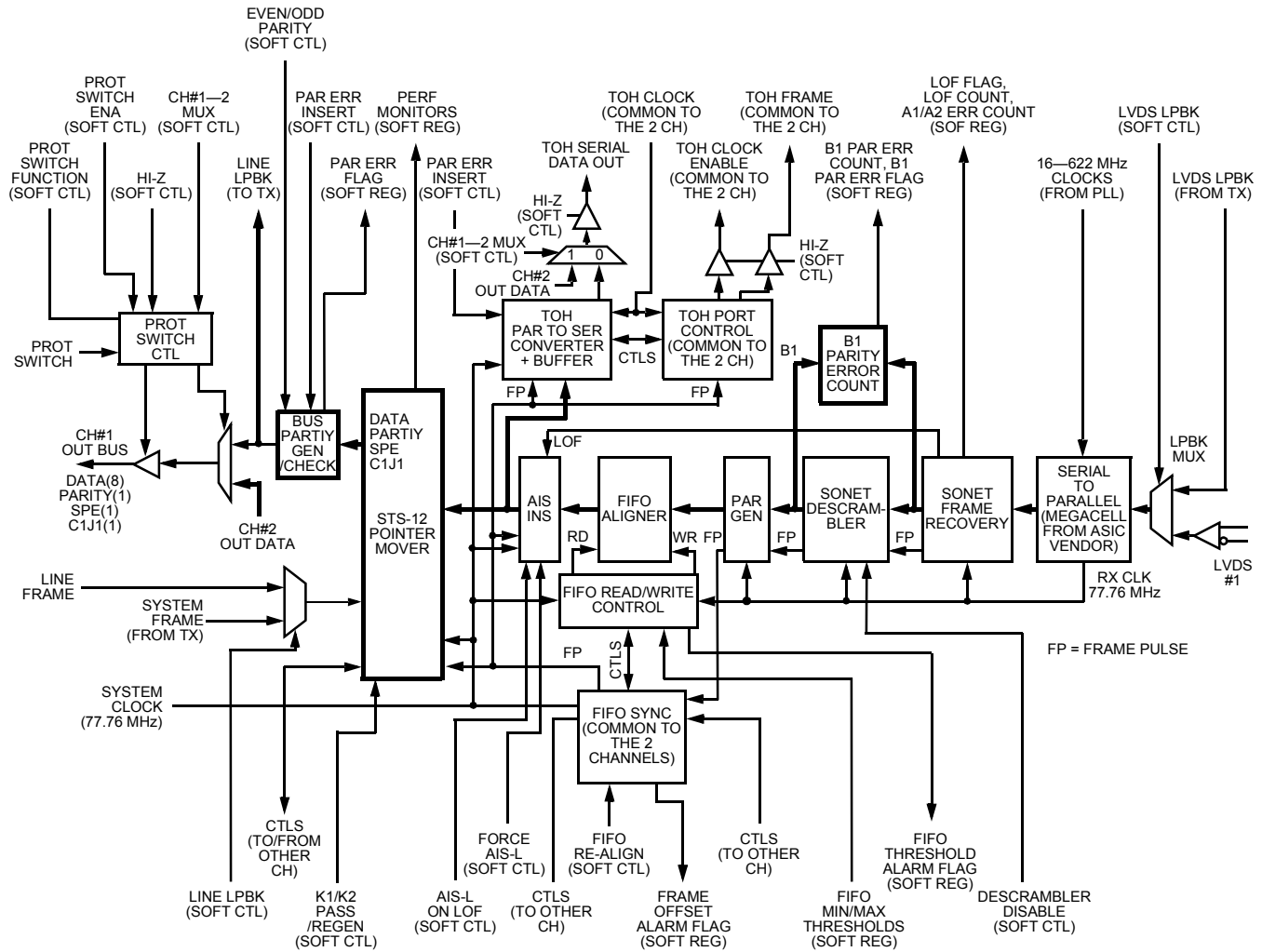
Figure 8. Receiver Block
